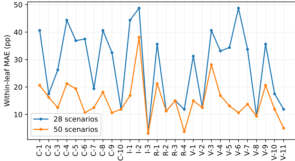
SR
