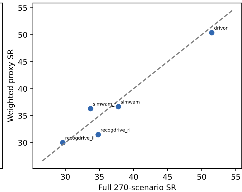
Frozen holdout: SR, MAE=1.70 pp
