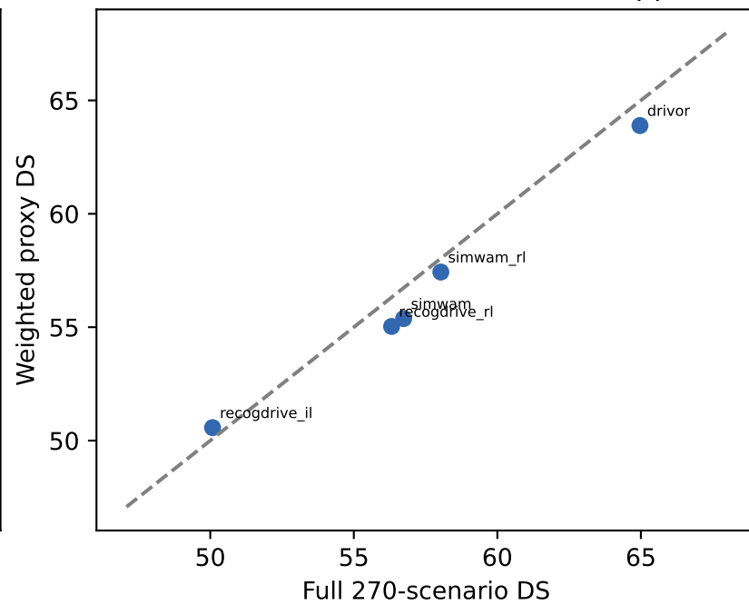
Frozen holdout: DS, MAE=0.96 pp
