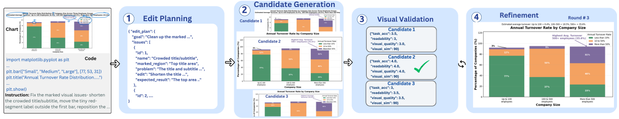
Figure 4: VisEditAgent framework. Given visualization code, a buggy, human-marked, or reference chart image, an instruction, and an edit intent, VisEditAgent plans the edit, generates candidate revisions, executes and renders them, validates the outputs, selects the best candidate, and refines it through iterative refinement rounds.
