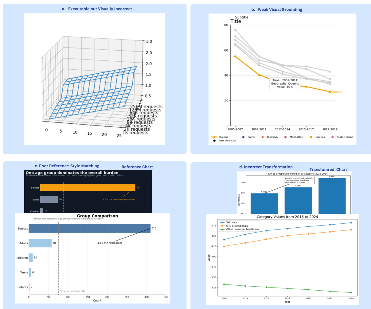
Figure 6: Error analysis examples showing that models often produce executable and visually plausible charts while missing the intended edit. (a) GPT-4o reduces clutter but the chart remains unreadable due to overlapping 1K–256M request labels. (b) GPT-4o fails to move the legend outside the line chart, leaving it over the plotted data. (c) InternVL-14B produces a clean chart but does not match the dark reference style. (d) Qwen3-VL-4B fails to transform the output into the reference visualization.
