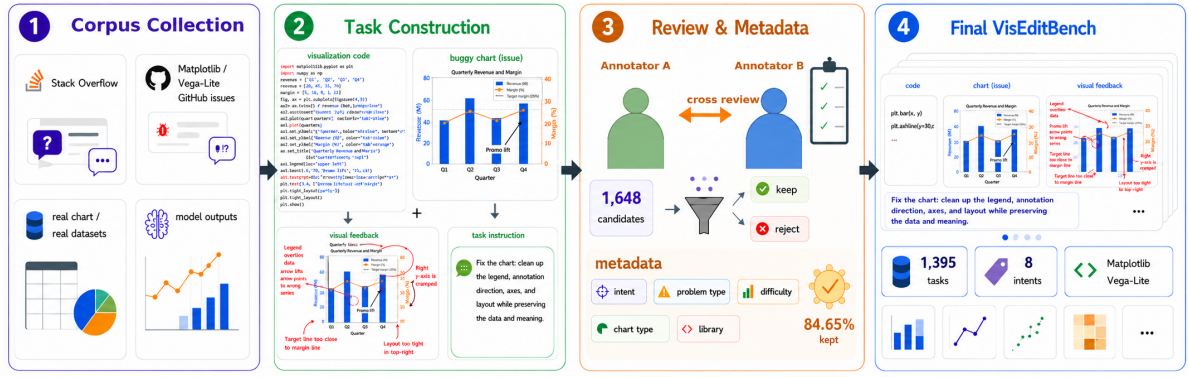
Figure 2: Overview of the VisEditBench construction pipeline. We collect real visualization issues and real-world chart/data examples, construct multimodal editing tasks, cross-review candidates for quality, and retain the final benchmark with metadata on editing intents, problem types, chart types, and visualization libraries.
