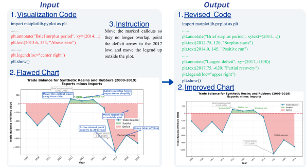
Figure 1: Overview of a VisEditBench task. Given visualization code, visual feedback or a reference chart, and a language instruction, the model must generate revised executable code that repairs or restyles the visualization while preserving the underlying data semantics.
