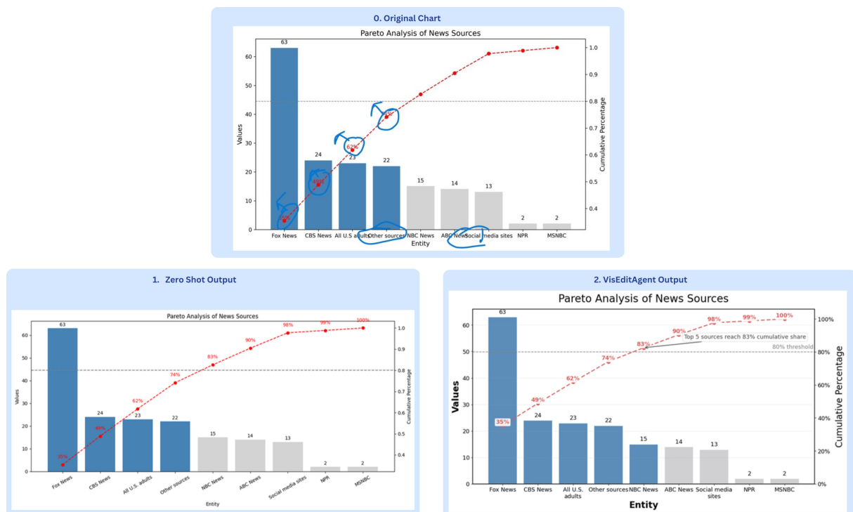
Figure 5: Qualitative example comparing GPT-4o zero-shot with GPT-4o + VisEditAgent. The original chart contains crowded x-axis labels and poorly positioned cumulative-percentage annotations. The editing instruction asks the model to improve label/annotation readability and spacing while preserving the chart semantics. Although GPT-4o zero-shot produces executable code, it only partially addresses these issues, whereas VisEditAgent produces a cleaner chart with better-positioned annotations and more readable labels.
