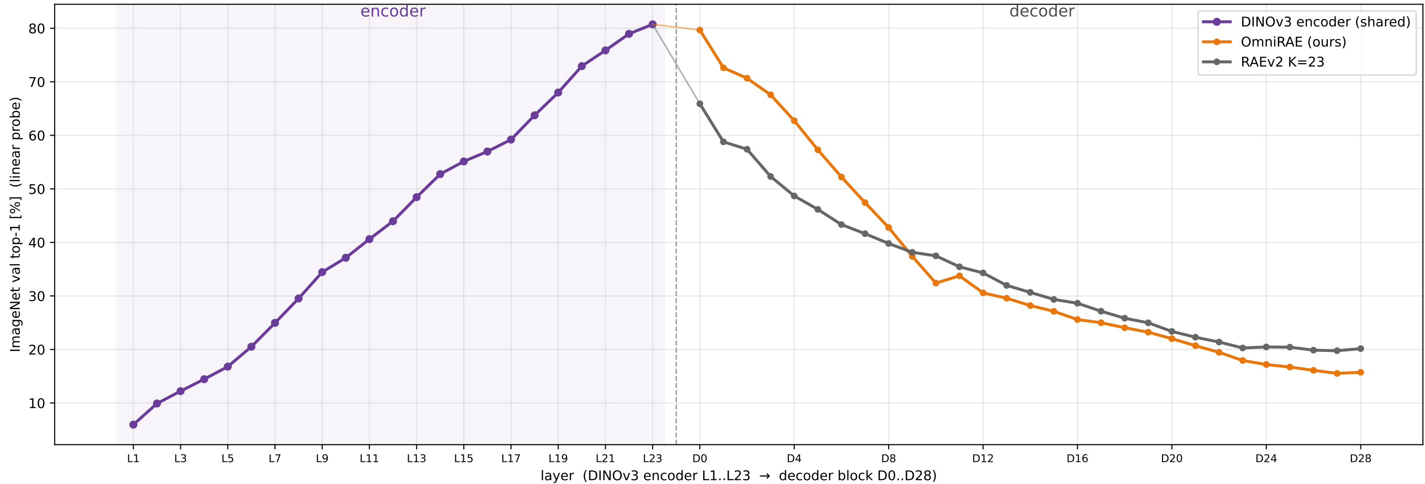
Semantic content through encoder then decoder (linear probe, 40/10 per class)
