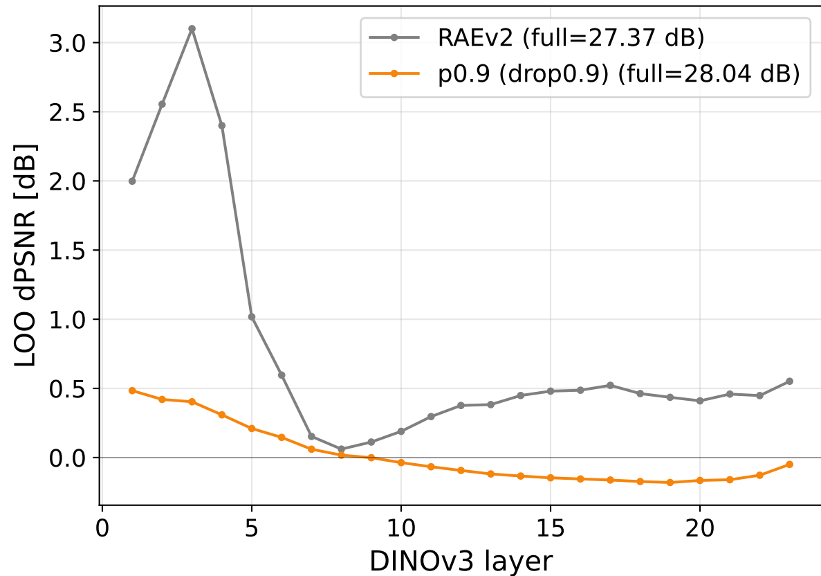
Leave-one-out reliance dPSNR = PSNR(all) - PSNR(all\ but\ i)
