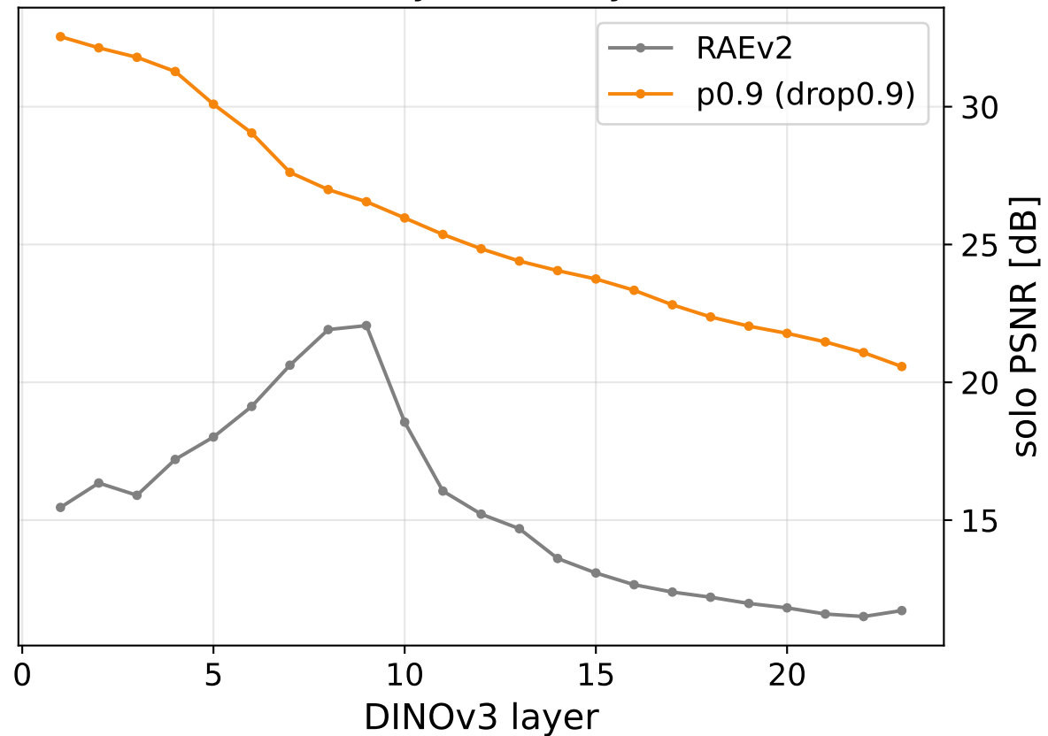
Solo sufficiency PSNR(layer\ i\ alone)
