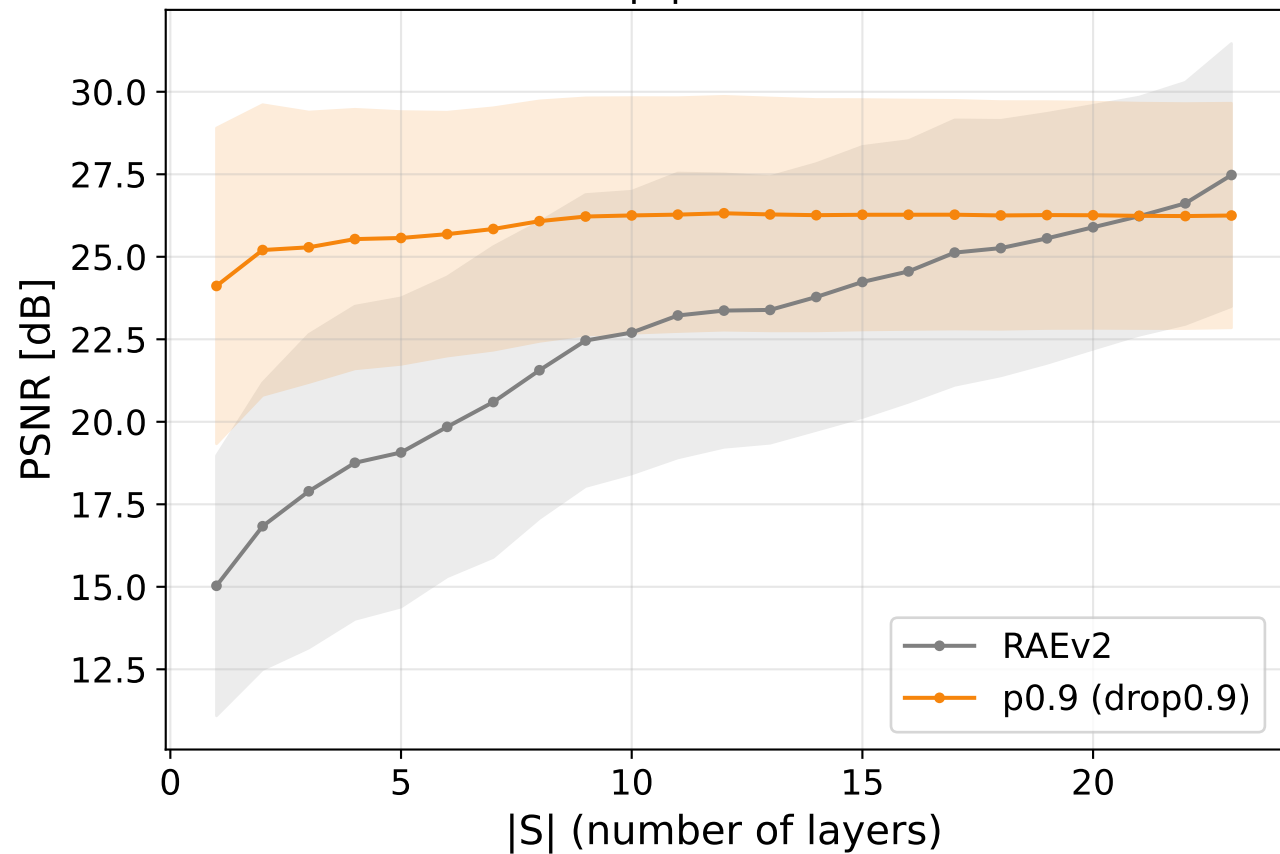
Value v(S) = \text{PSNR} vs |S| (line = mean, band = \pm std)
