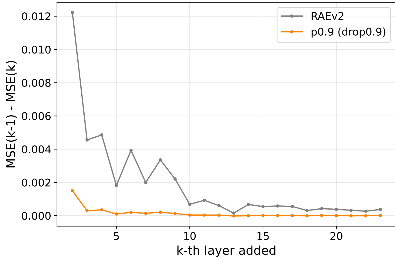
Marginal MSE reduction [MSE domain] (scale-dependence check)
