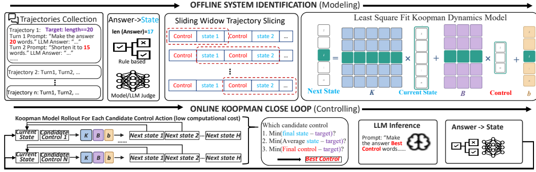
Figure 1: Overview of KOMPAS. Top, offline identification: recorded trajectories are mapped by the verifier V to readings, a sliding window forms the state s_t , and the affine Koopman model is fit by least squares. Bottom, online closed loop: candidate commands c_t are rolled forward through the model, scored against the reference r , and the best one is sent through the prompting protocol as u_t ; the next reading is shifted into the state and the selection repeats.
