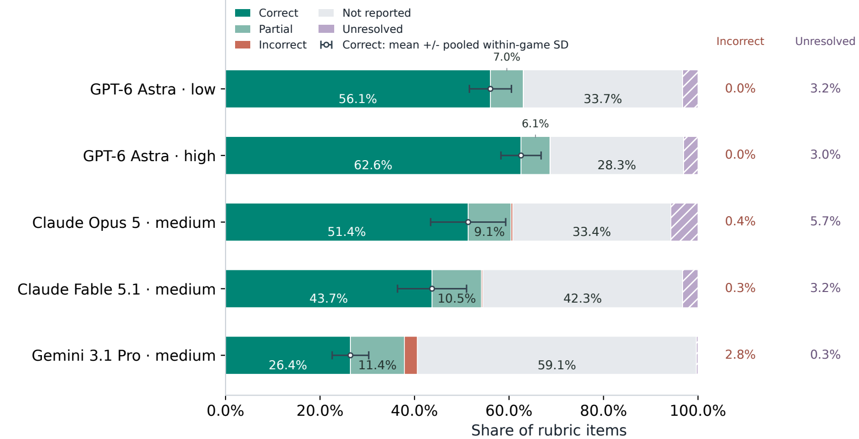
Core facts
