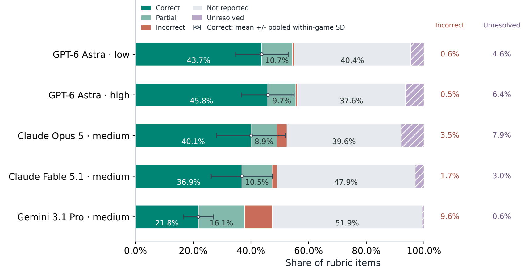
Core connections
