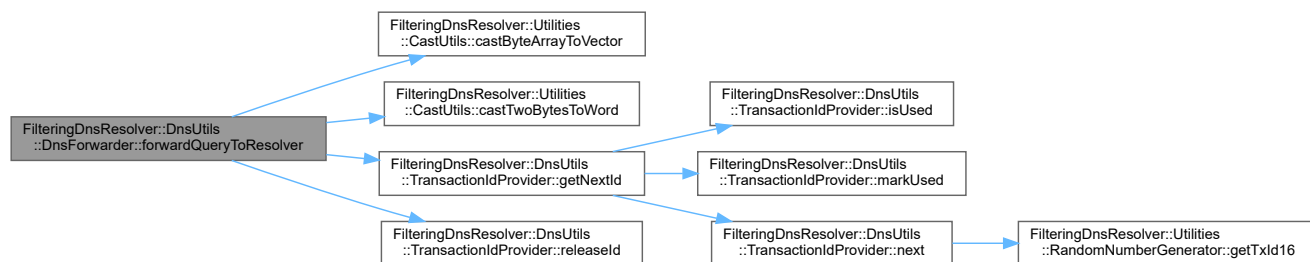
Obrázek 9: Call graph metody DnsUtils::DnsForwarder::forwardQueryToResolver()
