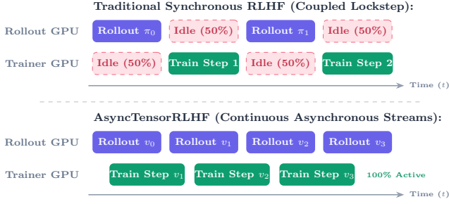
Figure 1: Execution schedule comparison: Synchronous RLHF incurs massive idle bubbles (50% duty cycle waste), whereas AsyncTensorRLHF achieves continuous 100% GPU utilization through decoupled concurrent execution.
