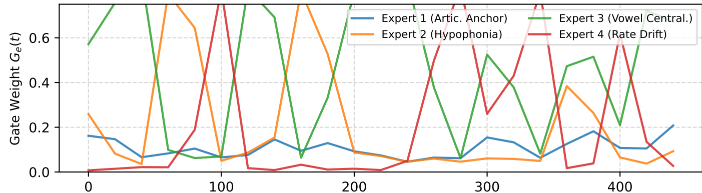
Severe Dysarthric Speaker (M02): Persistent Compensatory Expert Locking
