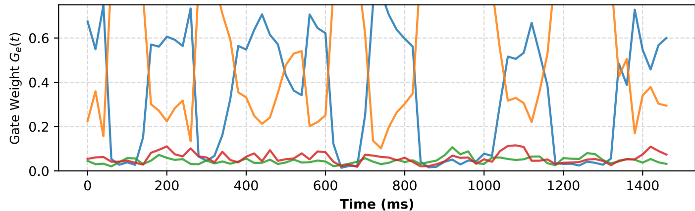
Severe Dysarthric Speaker (M02): Persistent Compensatory Expert Locking
