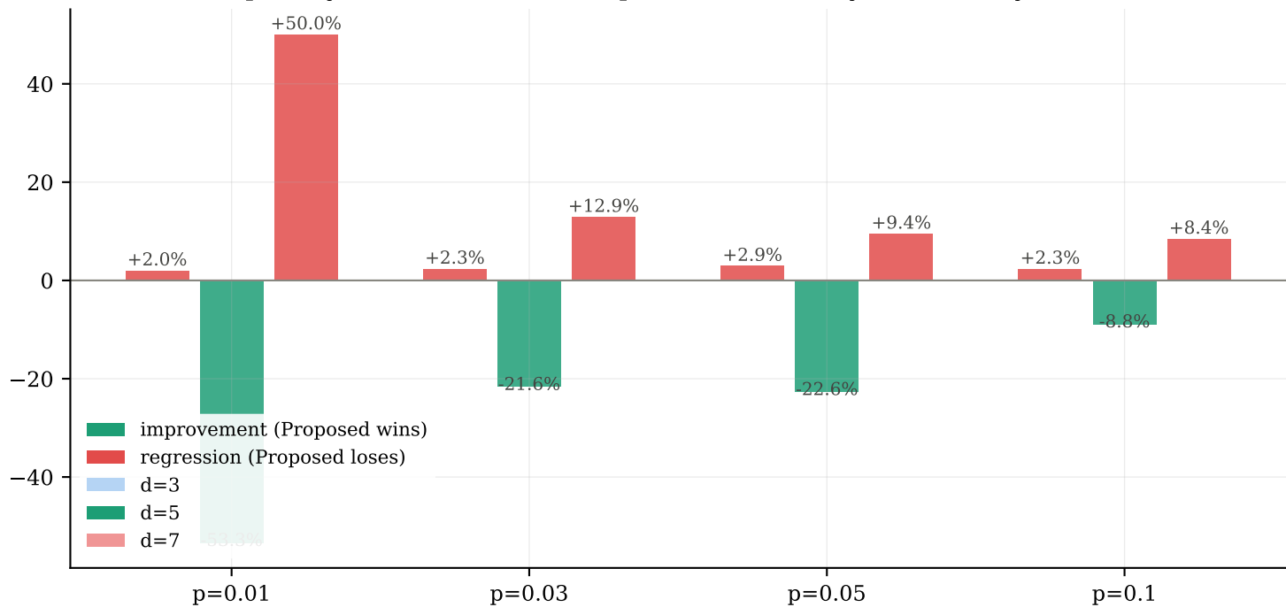
Gap analysis: ZX distillation improvement over syndrome-only baseline
