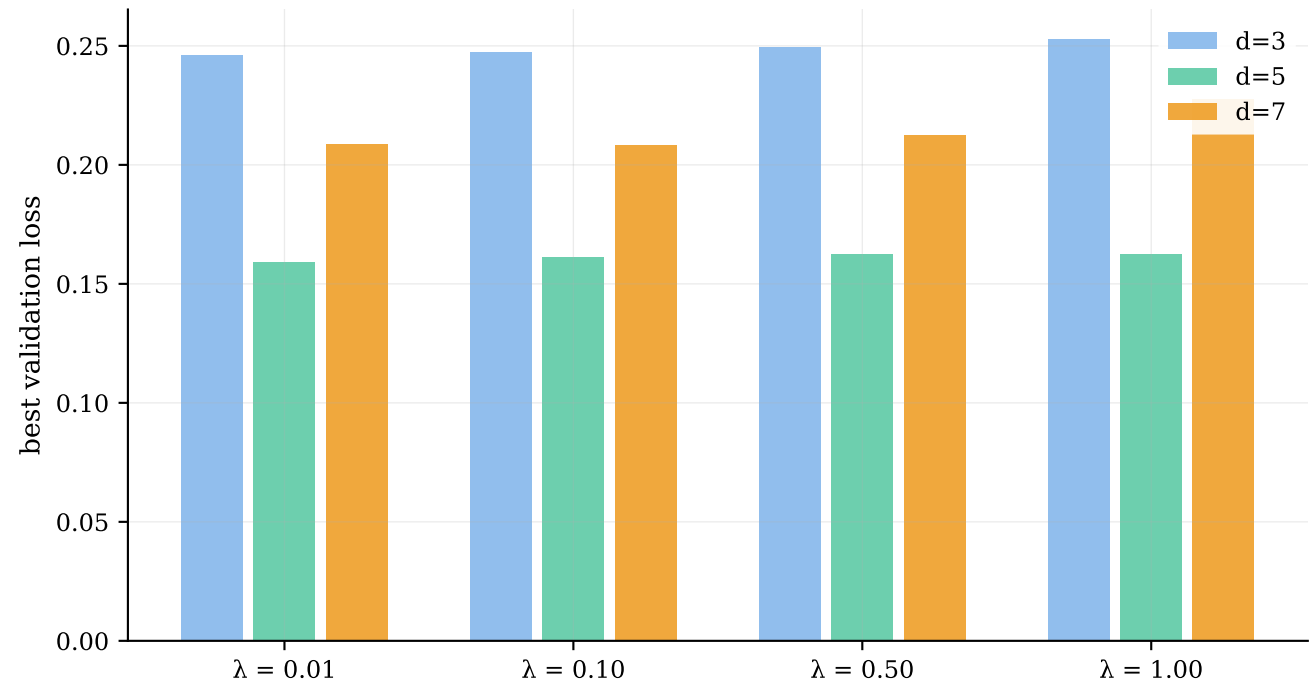
Lambda sweep: ProposedModel auxiliary loss weight
