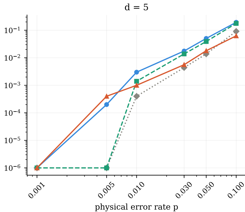
Logical error rate vs physical error rate
