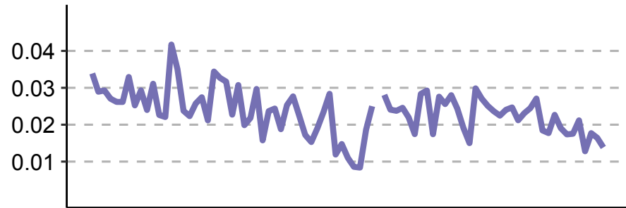
chr7:245000000-330000000
