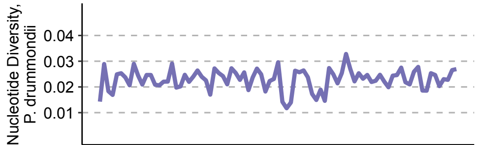
chr2:664000000-749000000
