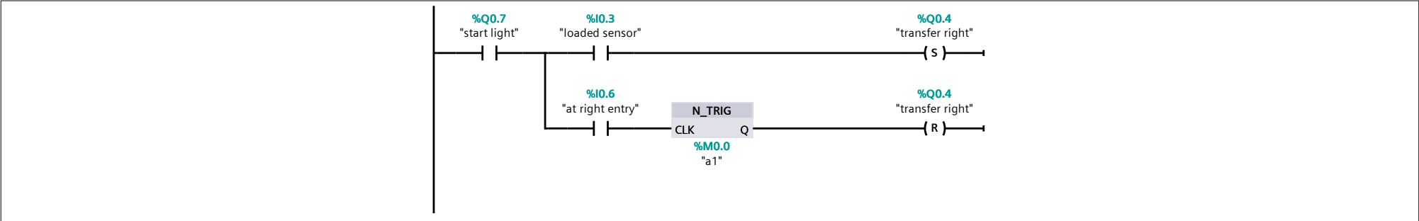
Network 6: right conveyor
