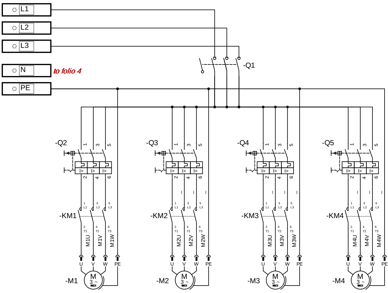
Feeder conveyor Entry conveyor Left conveyor Right conveyor
