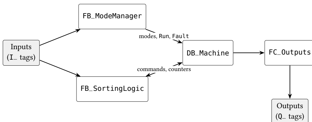
Figure 3.1. Data flow between the blocks of the program.
