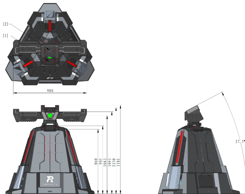
Figure 4-10 Base Foundation
