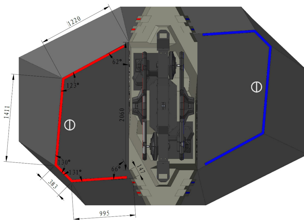
Figure 4-30 Assembly Zone Dimensions
