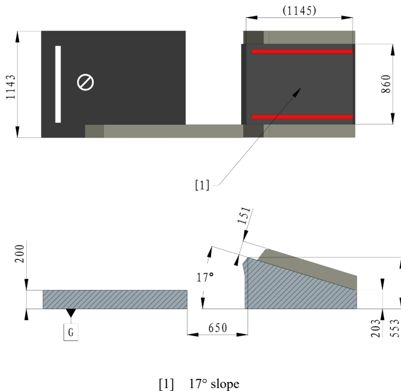
Figure 4-38 Launch Ramp
