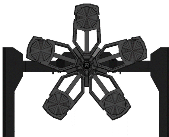
Figure 5-16 Power Rune in the Inactive State
