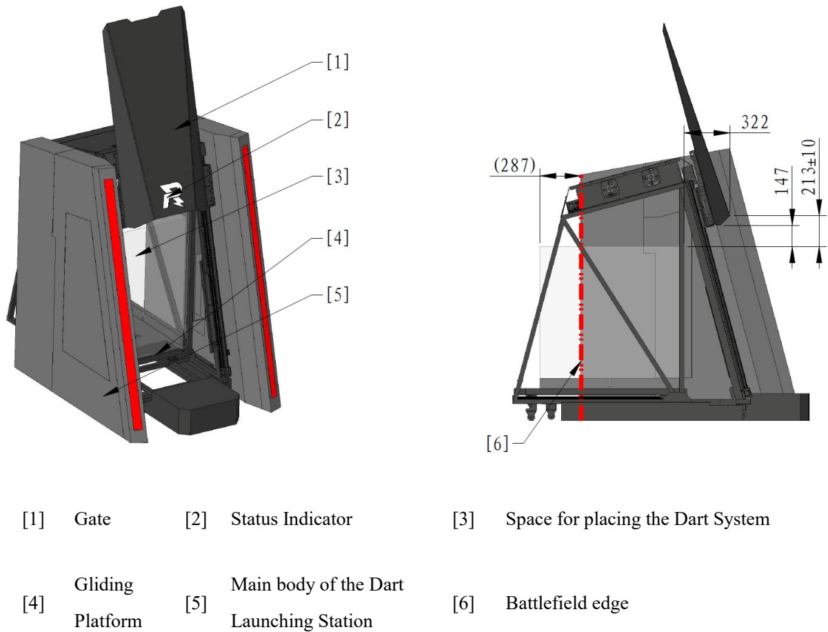
Figure 4-14 Dart Launching Station
