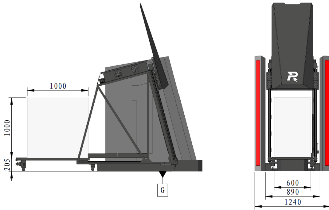
Figure 4-15 Gliding Platform Extension
