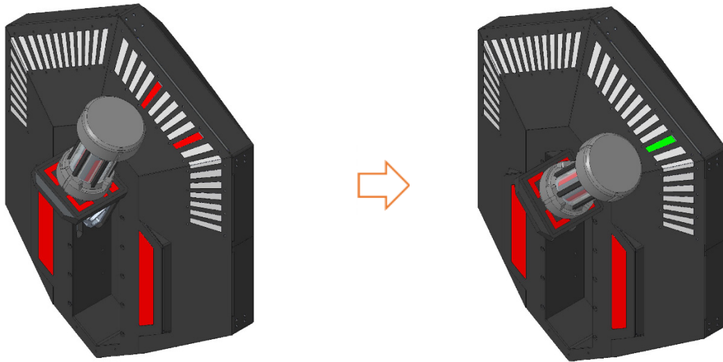
Figure 5-13 Step 5
