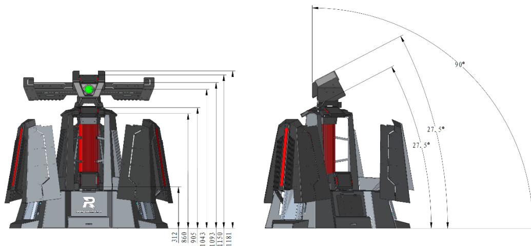
Figure 4-12 Expanded Base Protective Armor
