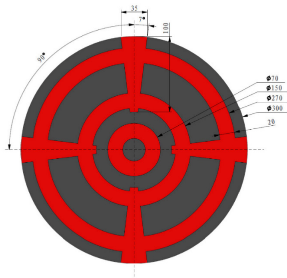
Figure 5-19 Power Rune in the Available State
