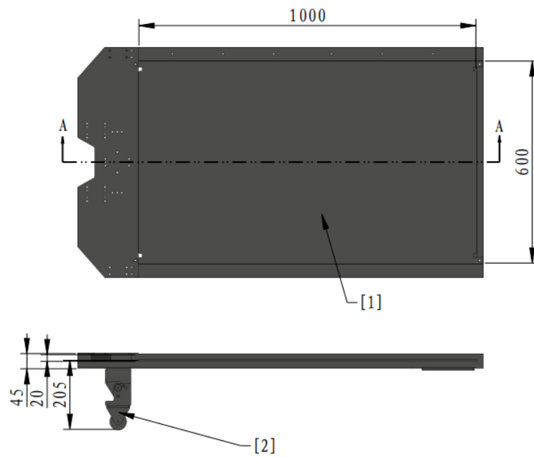
Figure 4-15 Gliding Platform Extension
