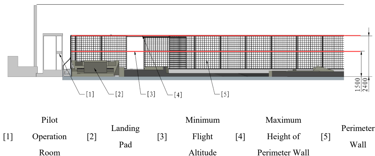
Figure 7-27 Flight Altitude Restrictions
