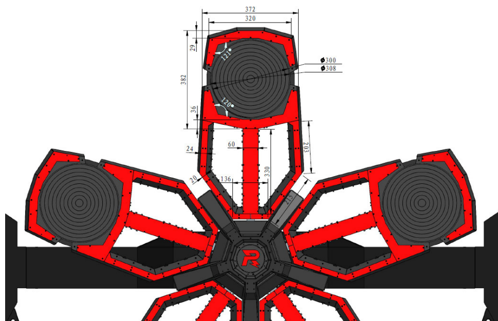
Figure 4-32 Power Rune Light Arm Dimensions
