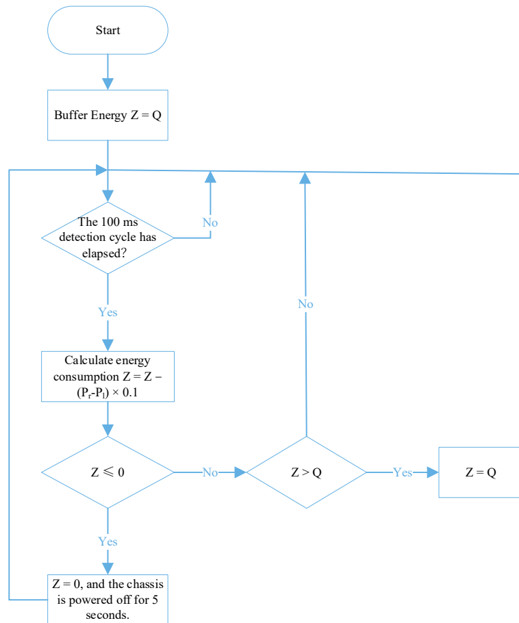
Figure 5-2 Robot Chassis Power Detection and Penalty for Exceeding Limit
