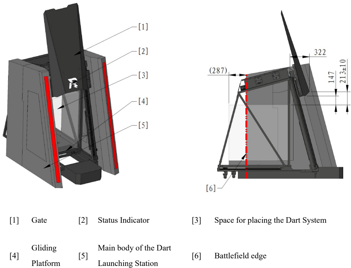
Figure 4-13 Dart Launching Station
