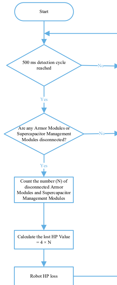
Figure 5-3 HP Loss Mechanism for Armor Module and Supercapacitor Management Module Disconnection
