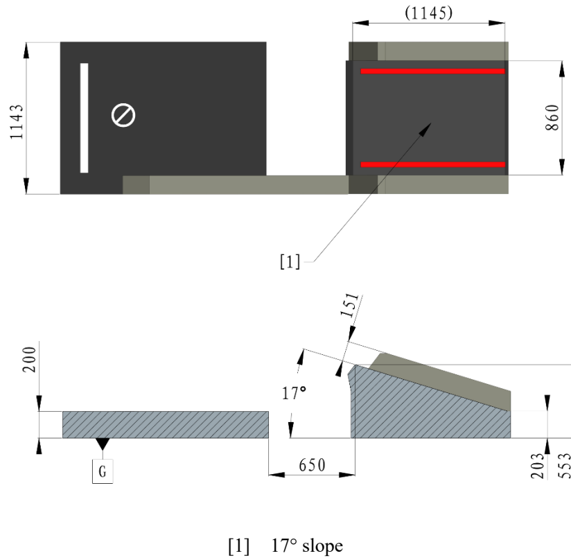
Figure 4-37 Launch Ramp
