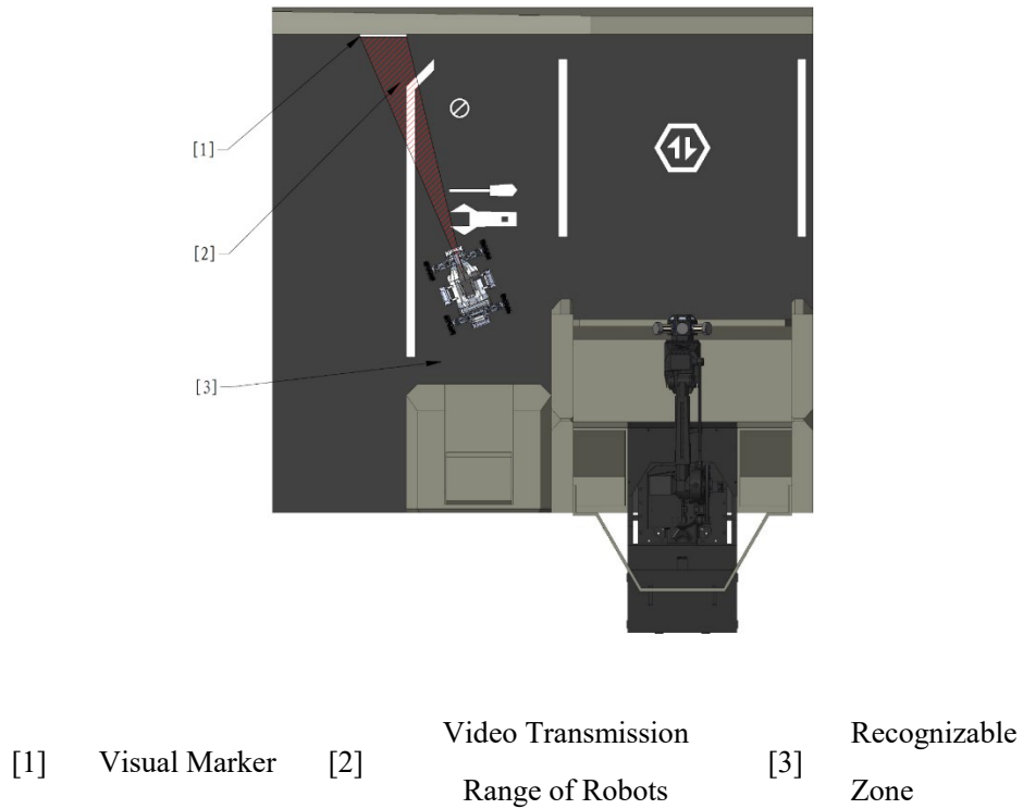
Figure 5-5 Relative Location of the Robot's Video Transmitter Module and Visual Marker
