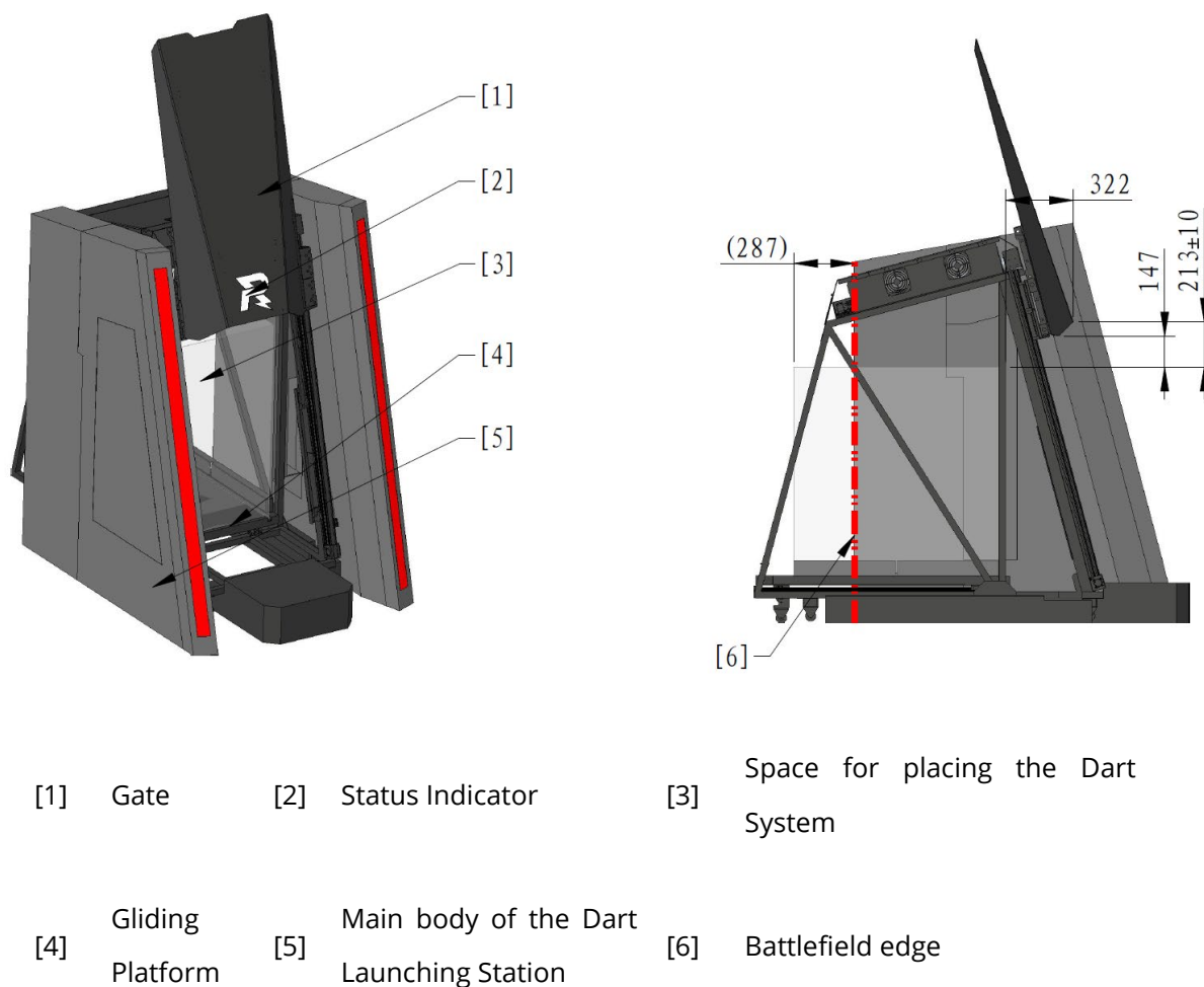
Figure 4-13 Dart Launching Station
