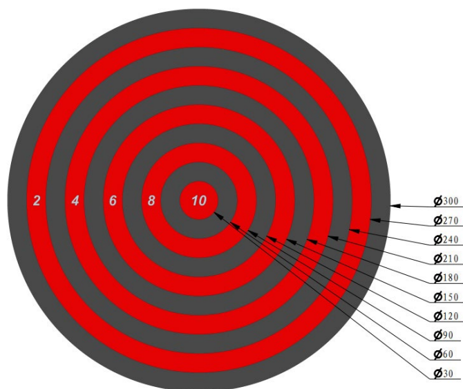
Figure 5-17 Power Rune Strike Area
