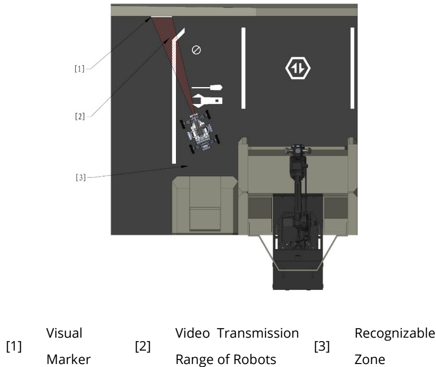
Figure 5-5 Relative Location of the Robot's Video Transmitter Module and Visual Marker
