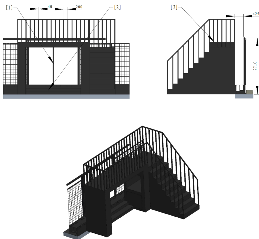
[1] Battlefield Entrance & Exit [2] Steps [3] Radar Foundation
