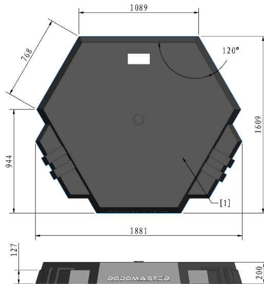
Figure 4-9 Base Foundation
