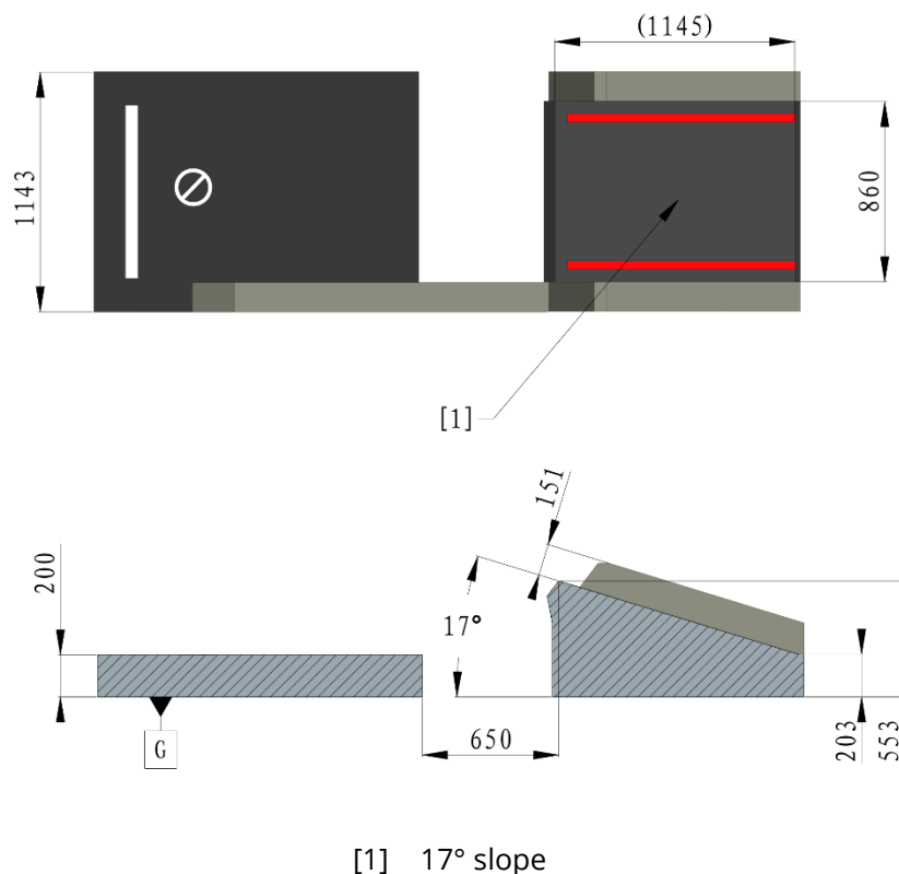
Figure 4-37 Launch Ramp
