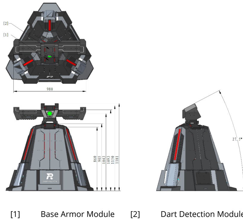
Figure 4-10 Closed Base Protective Armor
