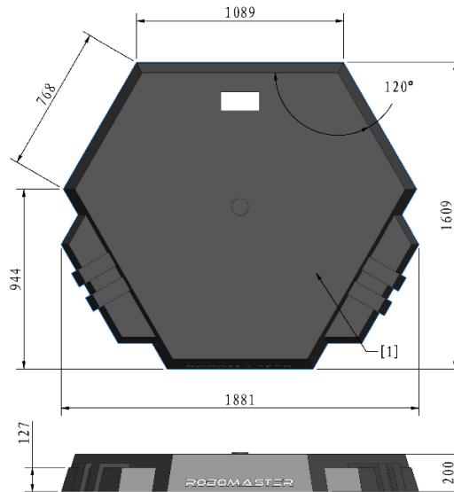
Figure 4-9 Base Foundation
