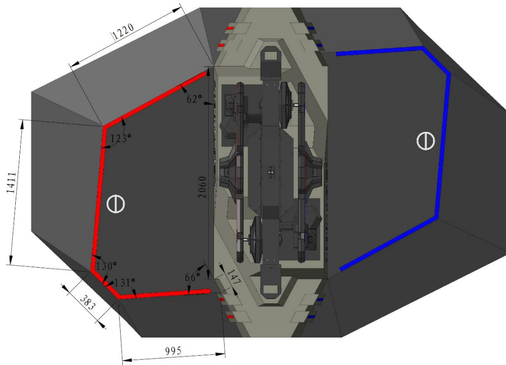
Figure 4-29 Assembly Zone Dimensions
