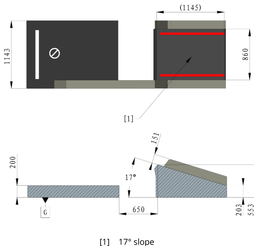
Figure 4-37 Launch Ramp
