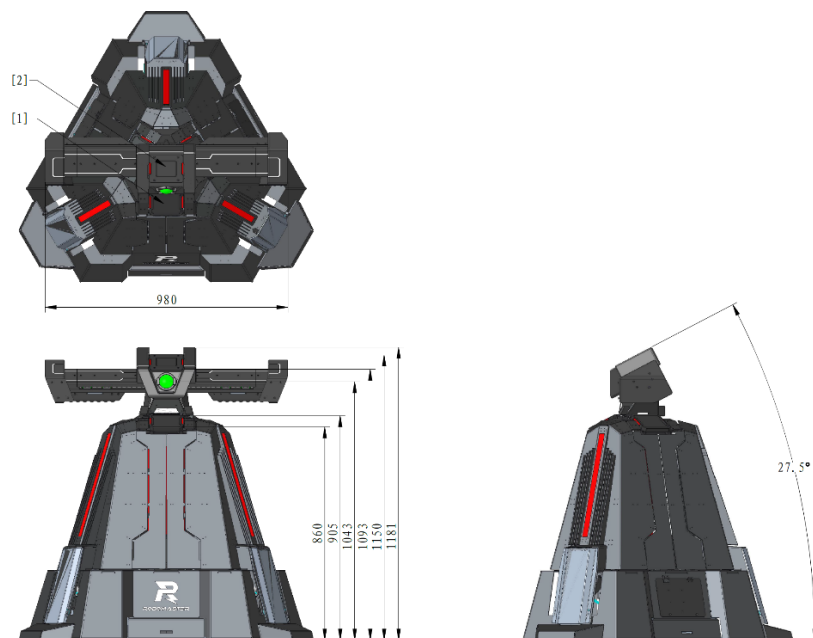
Figure 4-9 Base Foundation
