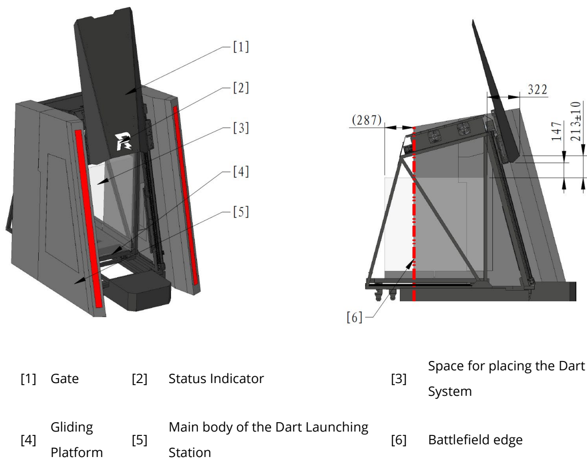
Figure 4-13 Dart Launching Station
