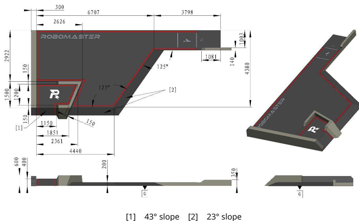
Figure 4-26 Trapezoid-Shaped Elevated Ground
