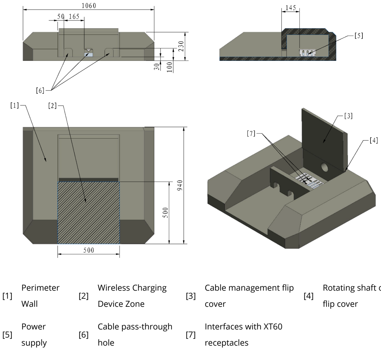
Figure 4-24 Wireless Charging Device
