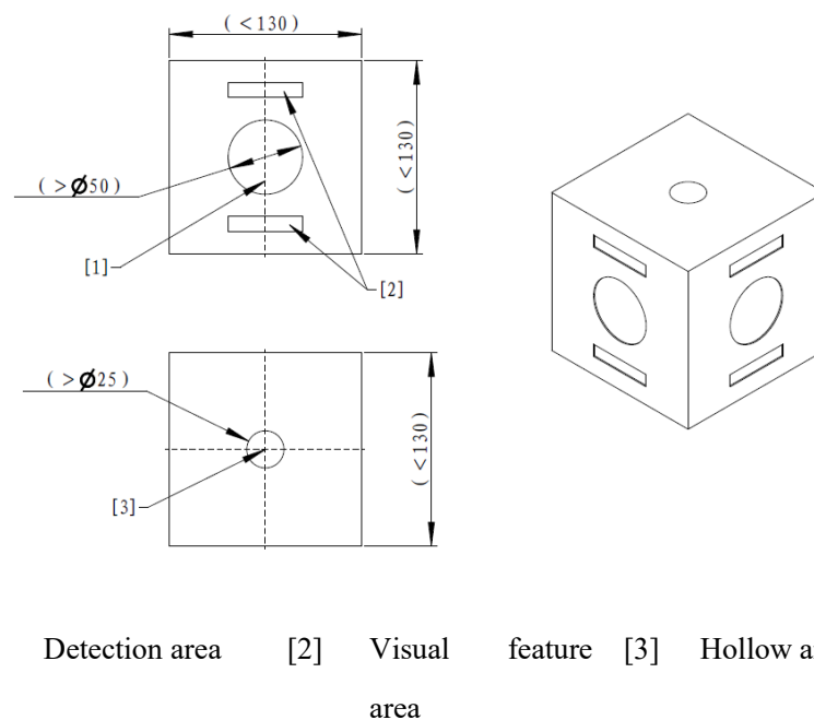
Figure 3-59 Laser Detection Module
