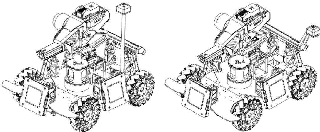
Figure 3-55 Mounting of UWB Positioning Module
