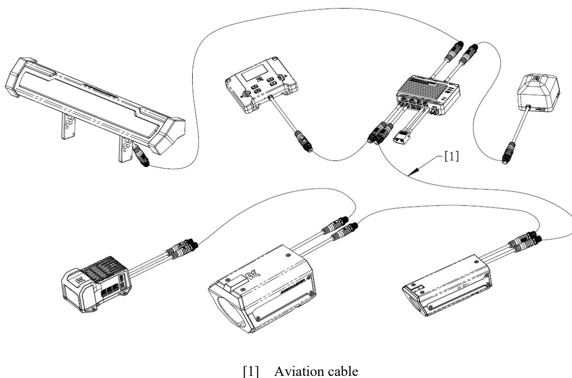
Figure 3-18 Wiring of Power Management Module
