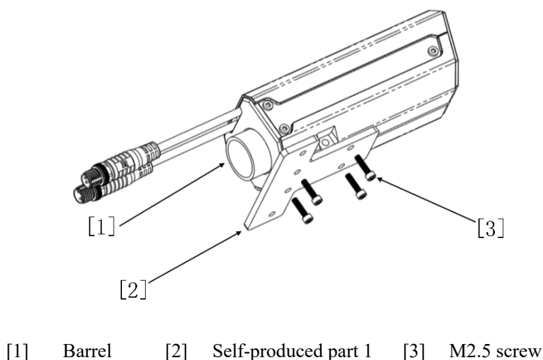
Figure 3-43 17mm Short Barrel Installation
