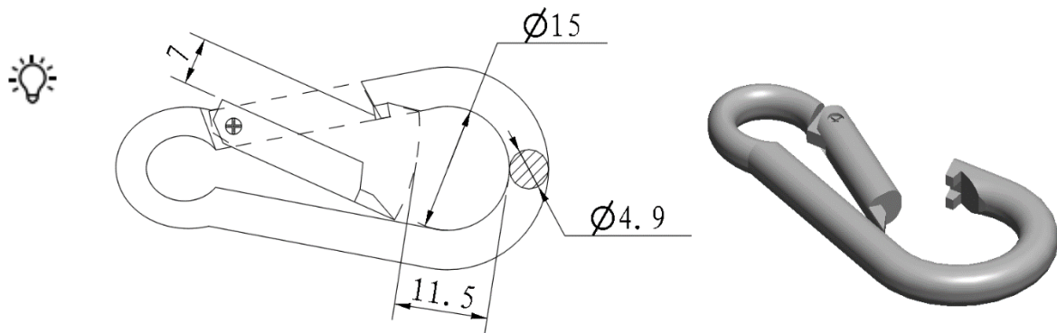
Figure 2-3 Aerial Safety Rope Hook Dimensions
