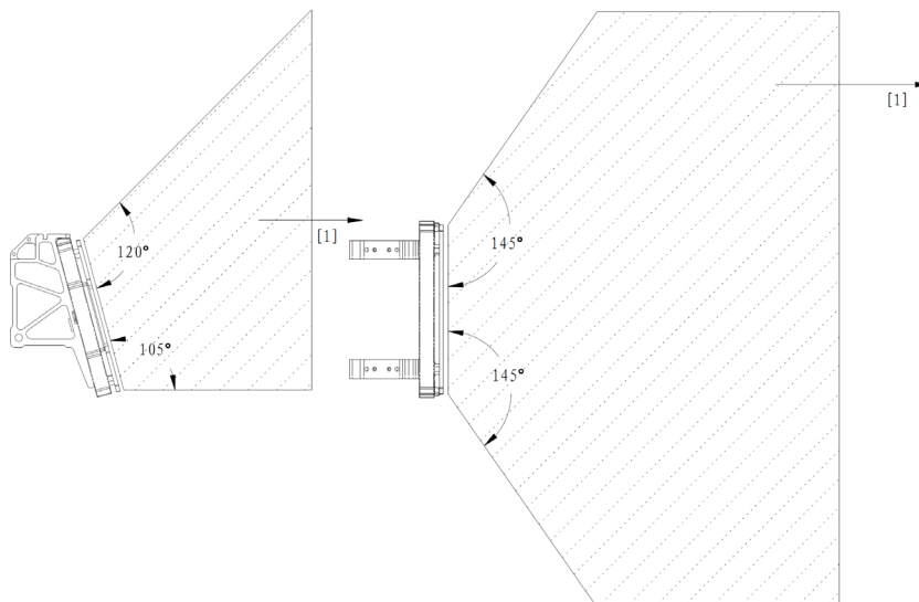
Figure 3-34 Mounting Specifications for Armor Module
