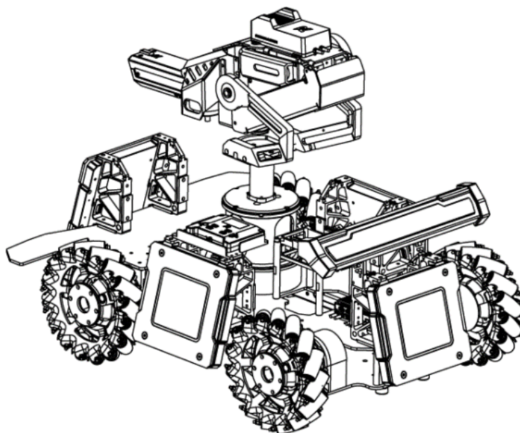
Figure 3-20 Mounting of Light Indicator Module
