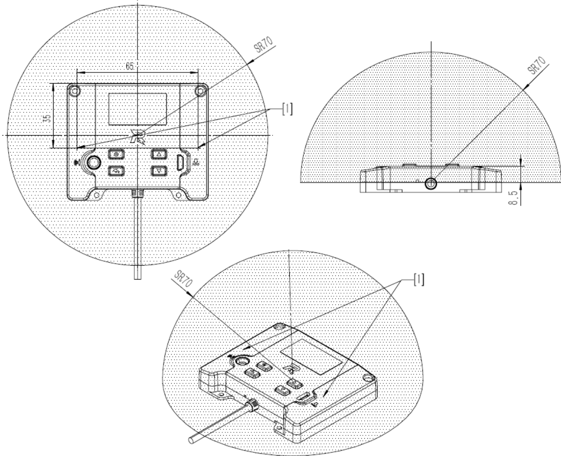
[1] Antenna's center
