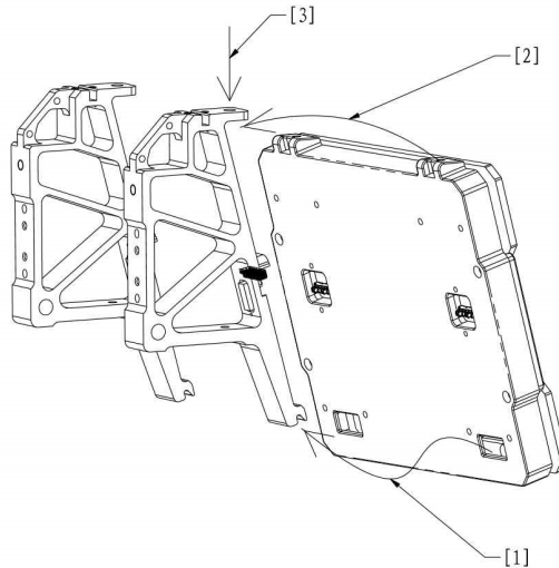
Figure 3-32 Armor Module Mounting
