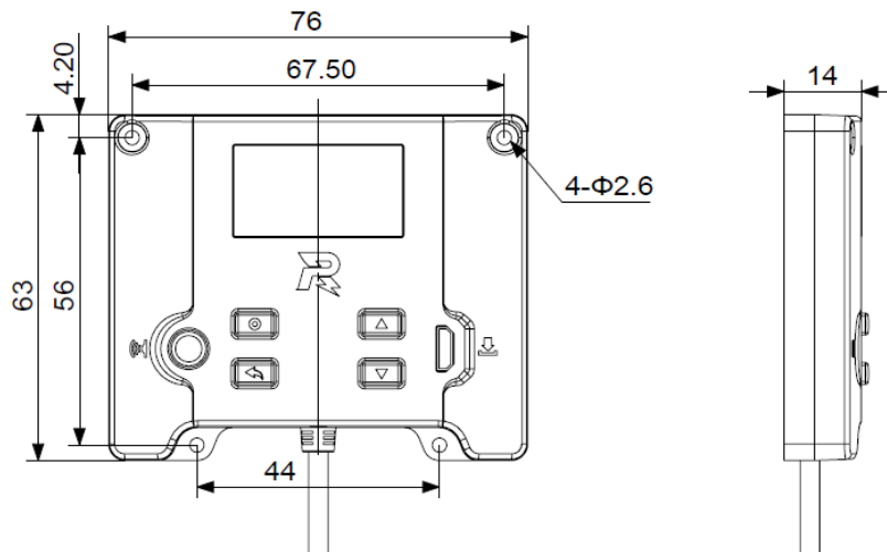
Figure 3-9 Main Control Module
