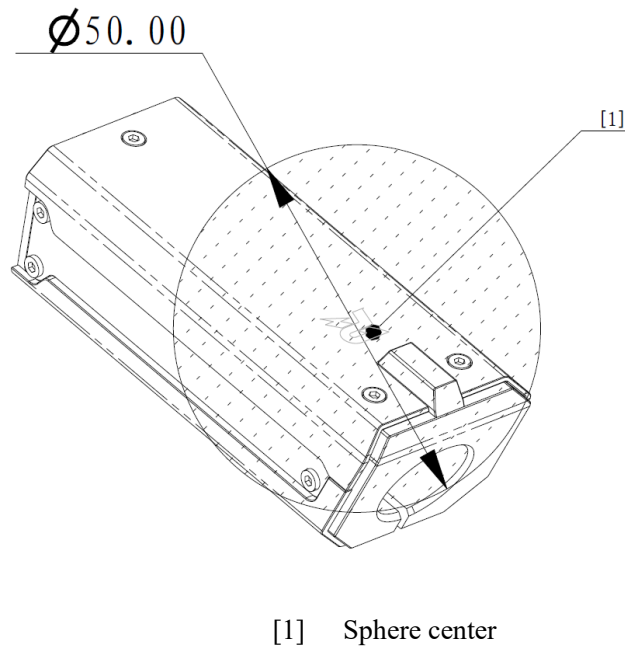
Figure 3-46 Mounting Specifications for Speed Monitor Module
