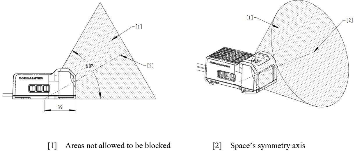
Figure 3-52 Prohibited Blockage Areas for Video Transmitter Module (Transmitter)
