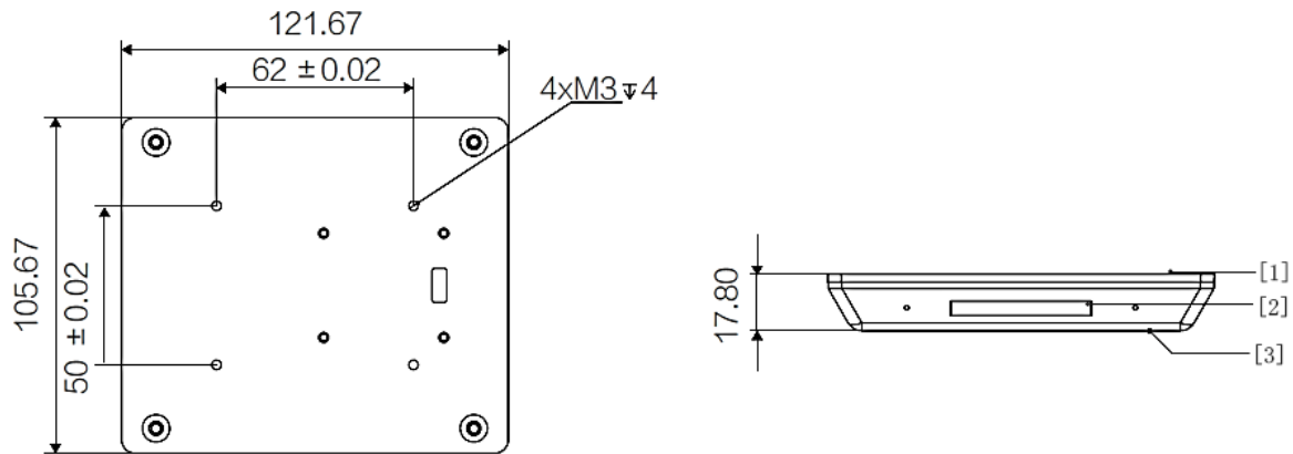
[1] Back [2] LED Indicator [3] Front
