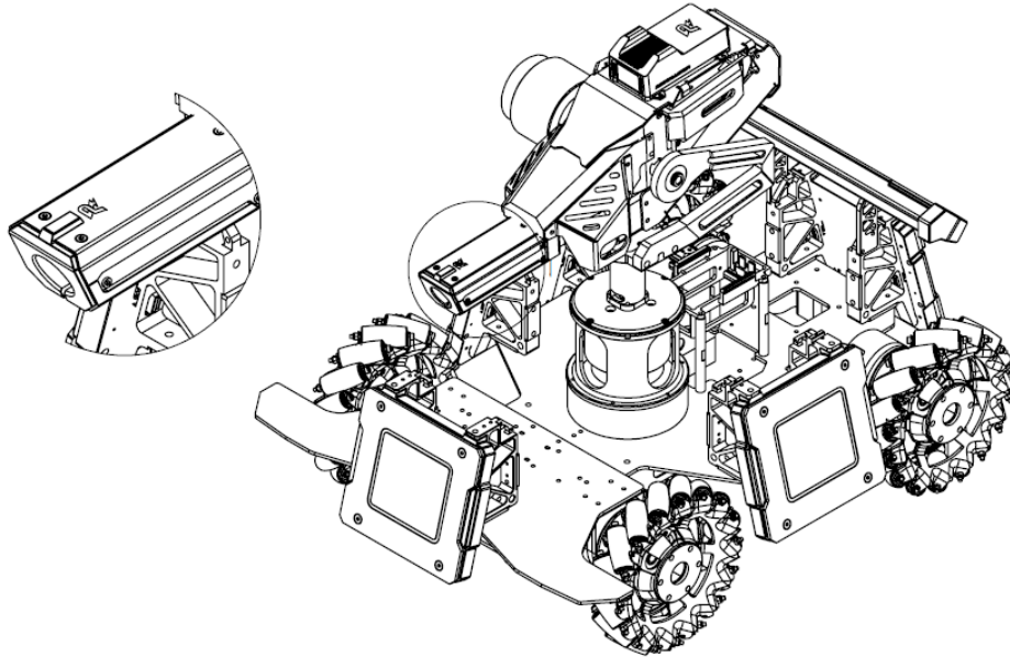
Figure 3-40 Speed Monitor Module Installation
