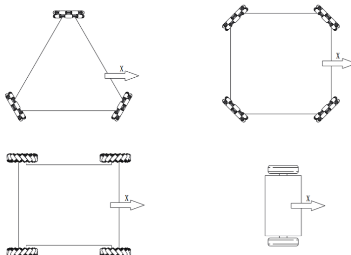
Figure 3-27 Graph of X-axis Orientation in Different Chassis Configurations of Robots
