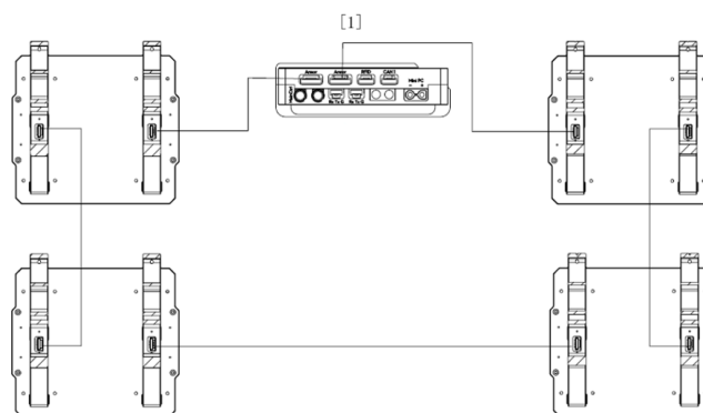
[1] Power Management Module
