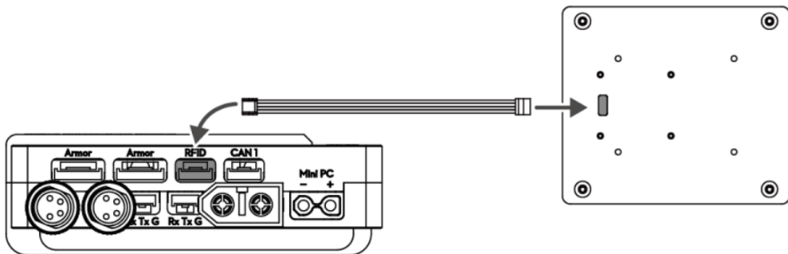
Figure 3-48 Wiring of RFID Interaction Module
