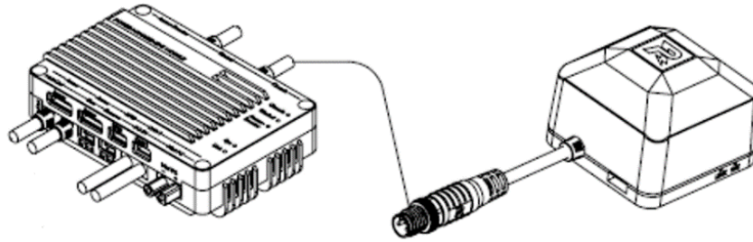
Figure 3-56 Wiring of UWB Positioning Module
