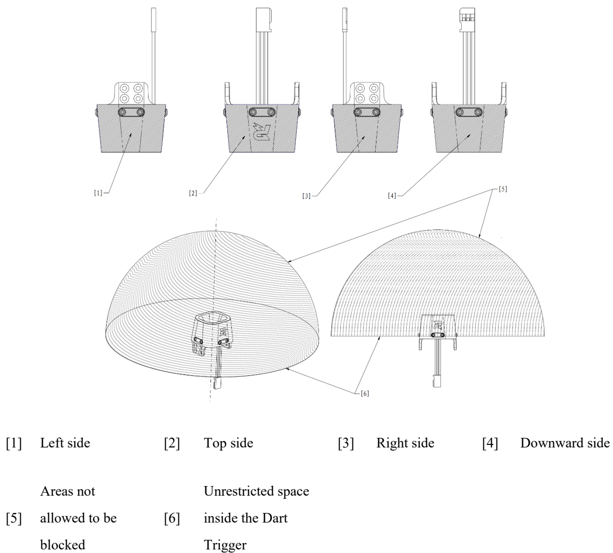
Figure 2-7 Prohibited Blockage Areas for Dart Trigger
