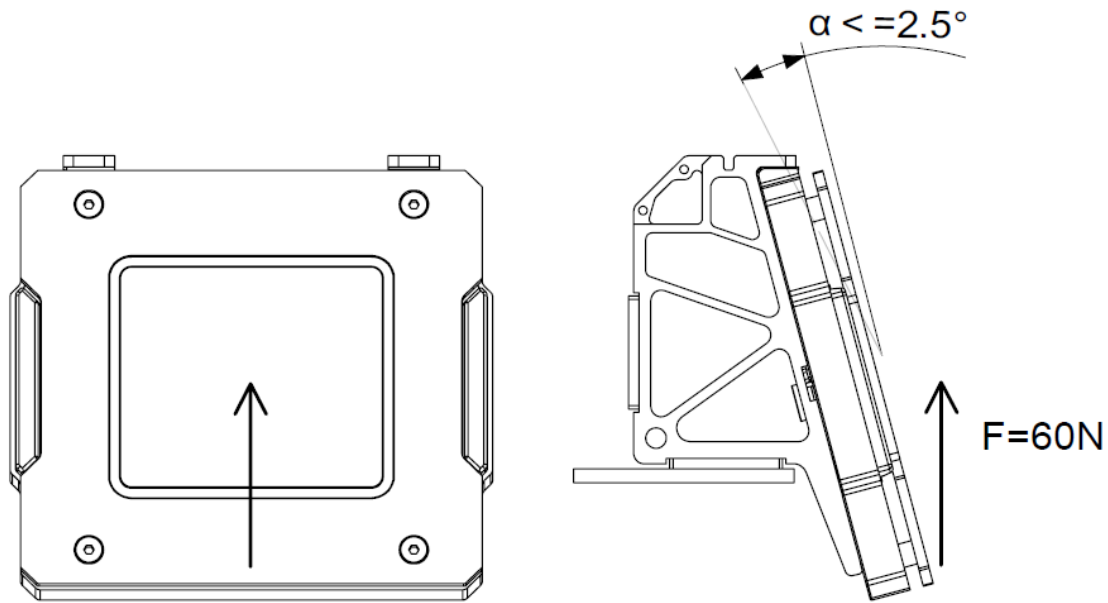
Figure 3-28 Forces on the Armor Module
