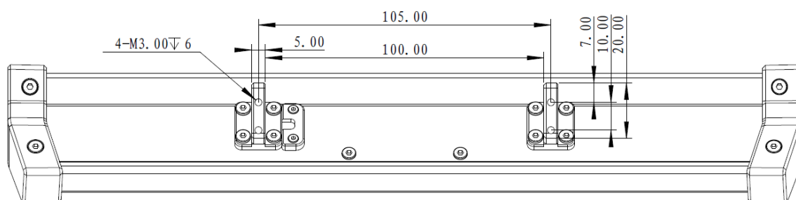
Figure 3-21 Bottom of the Light Indicator Module
