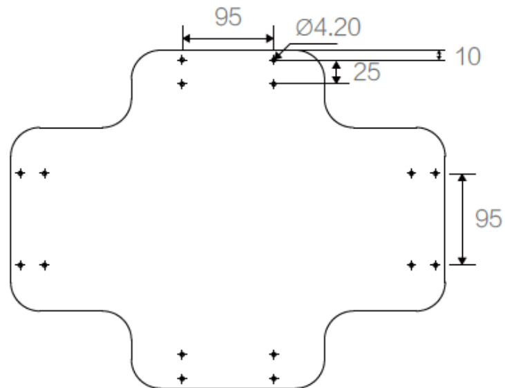
Figure 3-30 Chassis Reserved Holes
