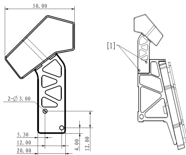
[1] Screw mounting positions
