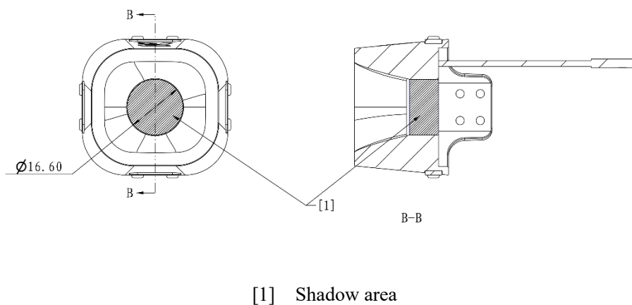
Figure 2-8 Internal Cavity of Dart Trigger
