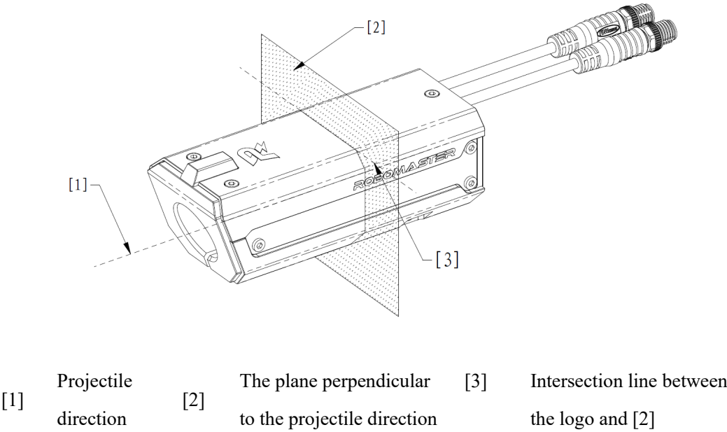
Figure 3-37 Speed Monitor Module Installation
