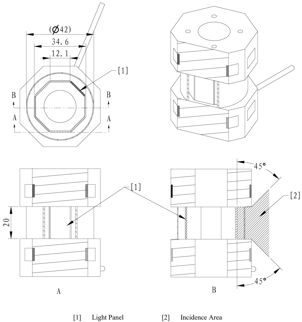
Figure 3-52 Laser Detection Module
