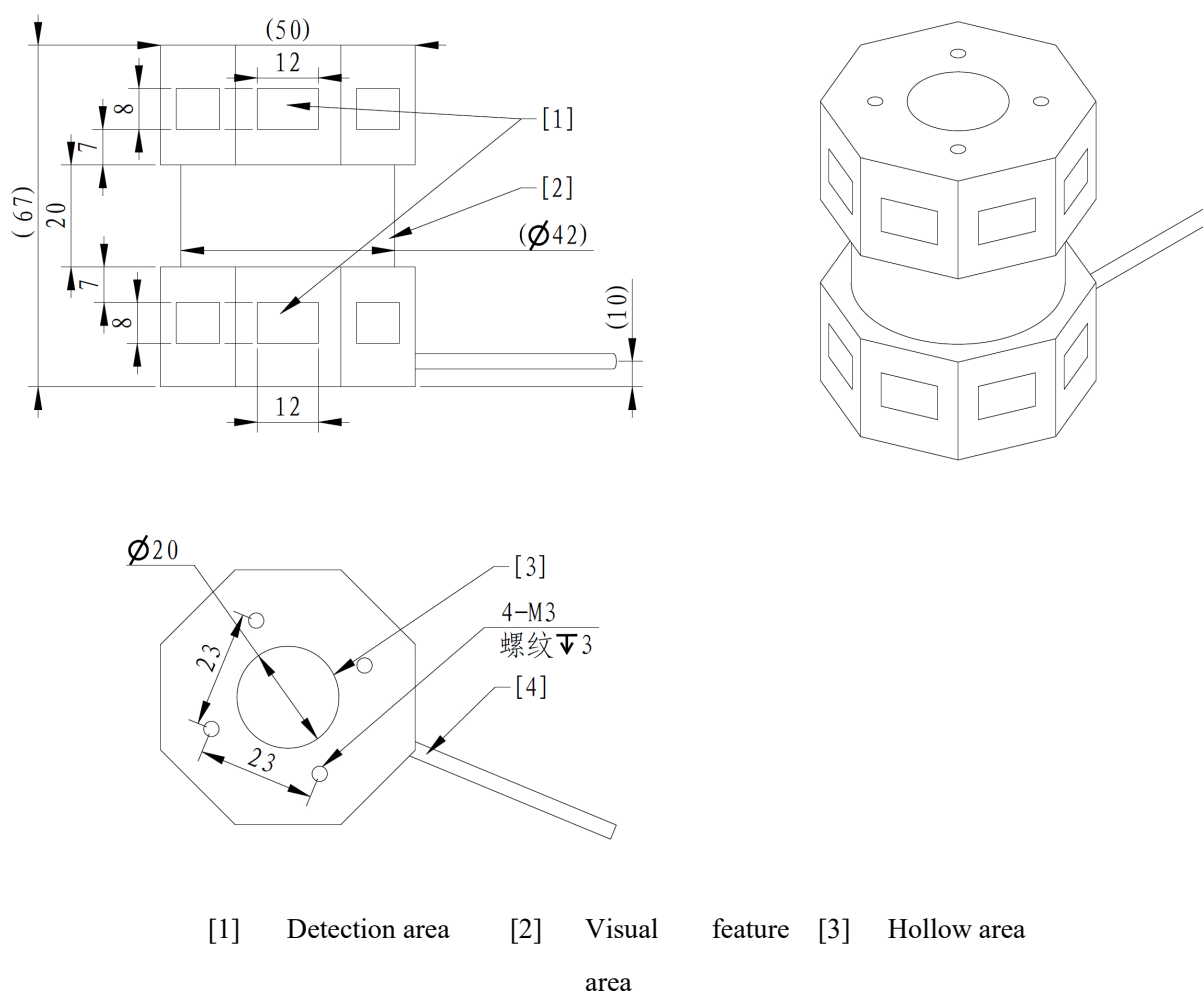
Figure 3-51 Laser Detection Module
