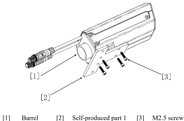
Figure 3-35 17mm Short Barrel Installation
