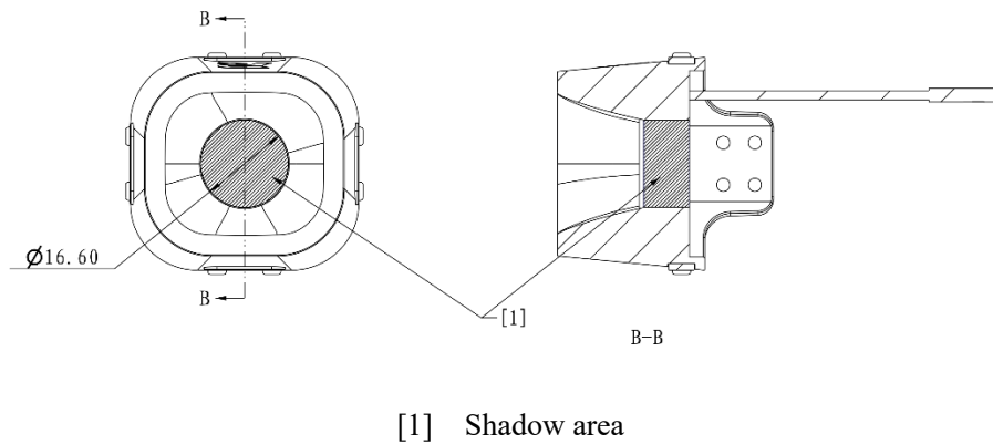
Figure 2-9 Internal Cavity of Dart Trigger
