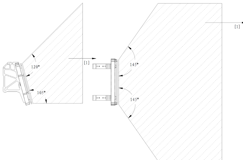
Figure 3-26 Mounting Specifications for Armor Module
