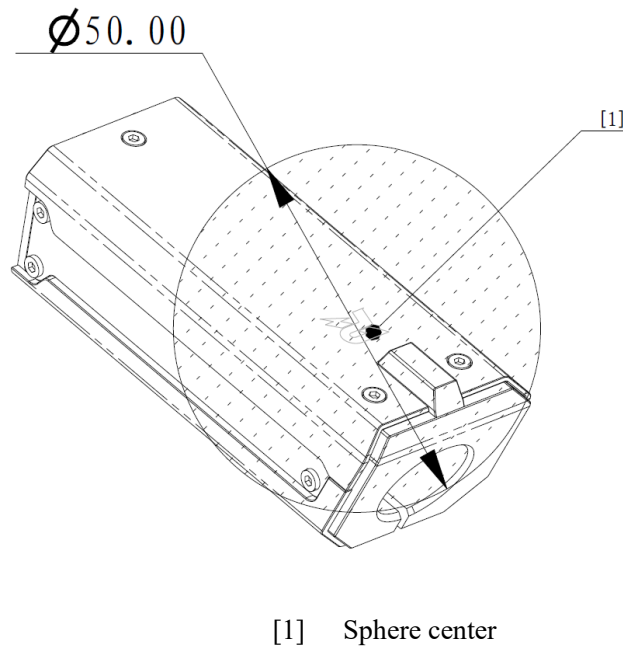
Figure 3-38 Mounting Specifications for Speed Monitor Module
