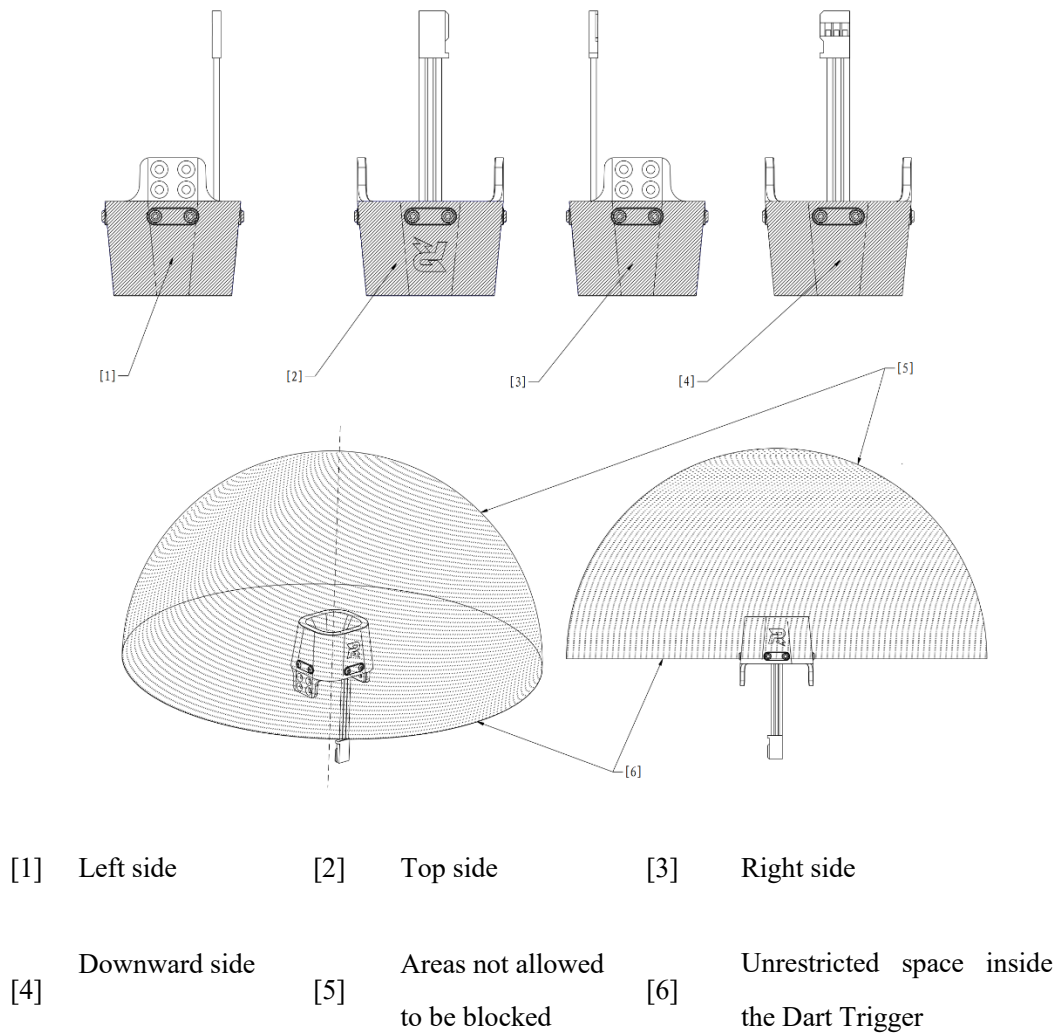
Figure 2-8 Prohibited Blockage Areas for Dart Trigger
