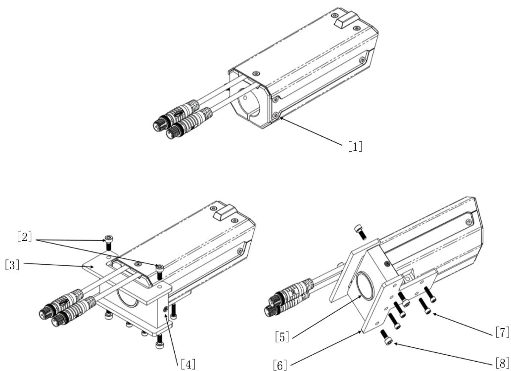
[1] M2.5 screw for securing LED Indicator
