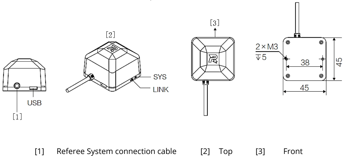
Figure 3-46 UWB Positioning Module
