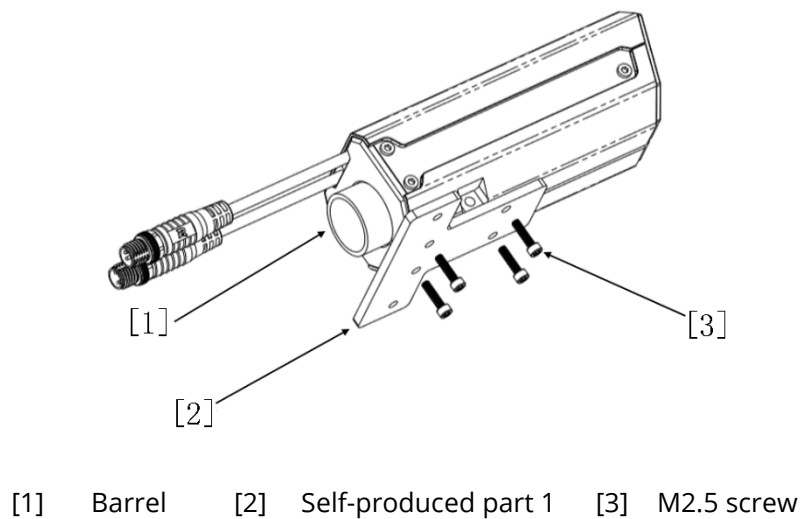
Figure 3-35 17mm Short Barrel Installation
