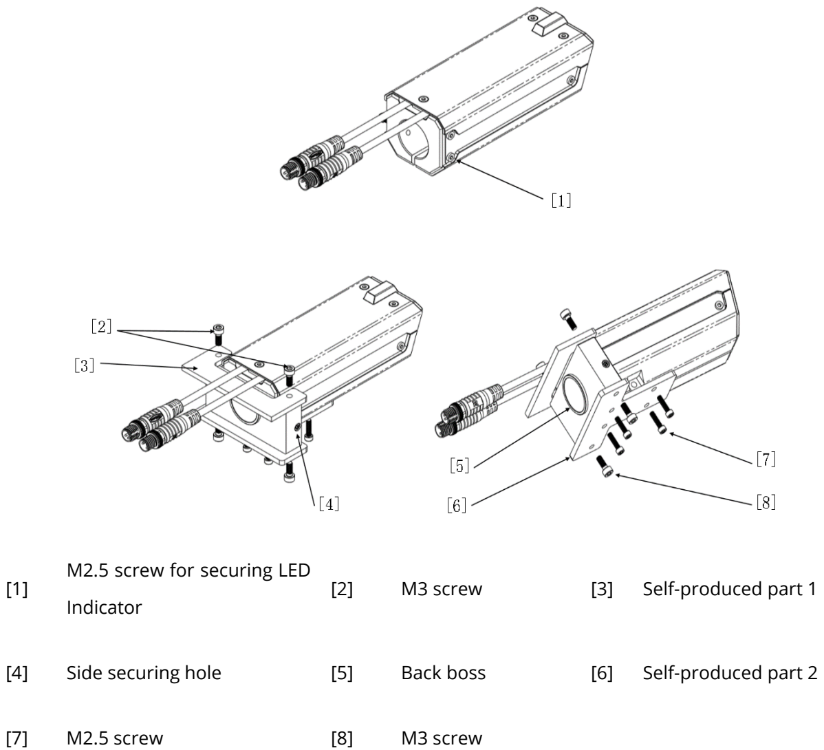
Figure 3-34 17mm Adapter Block Securing Method
