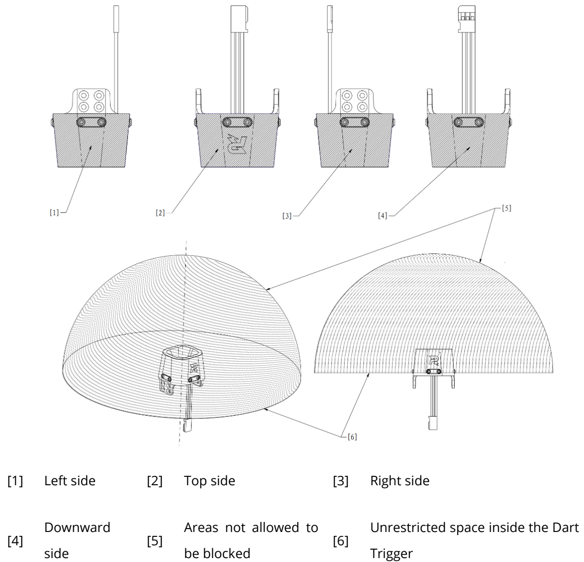
Figure 2-8 Prohibited Blockage Areas for Dart Trigger
