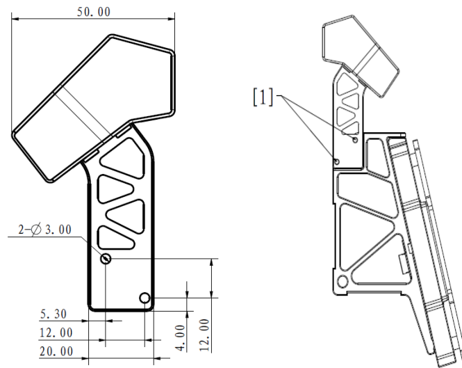
[1] Screw mounting positions
