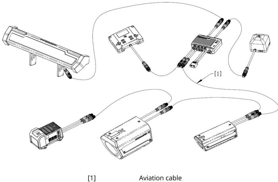
Figure 3-10 Wiring of Power Management Module
