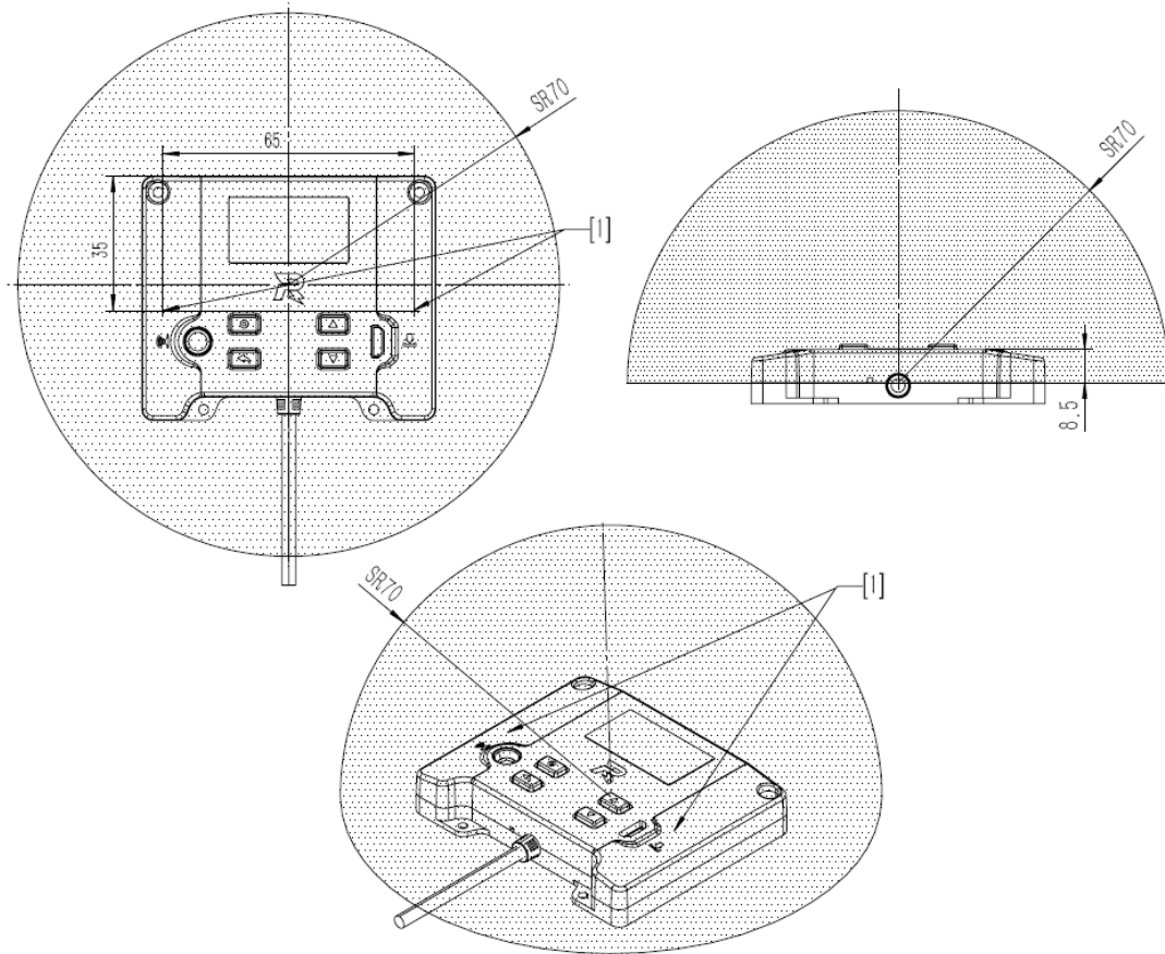
[1] Antenna's center
