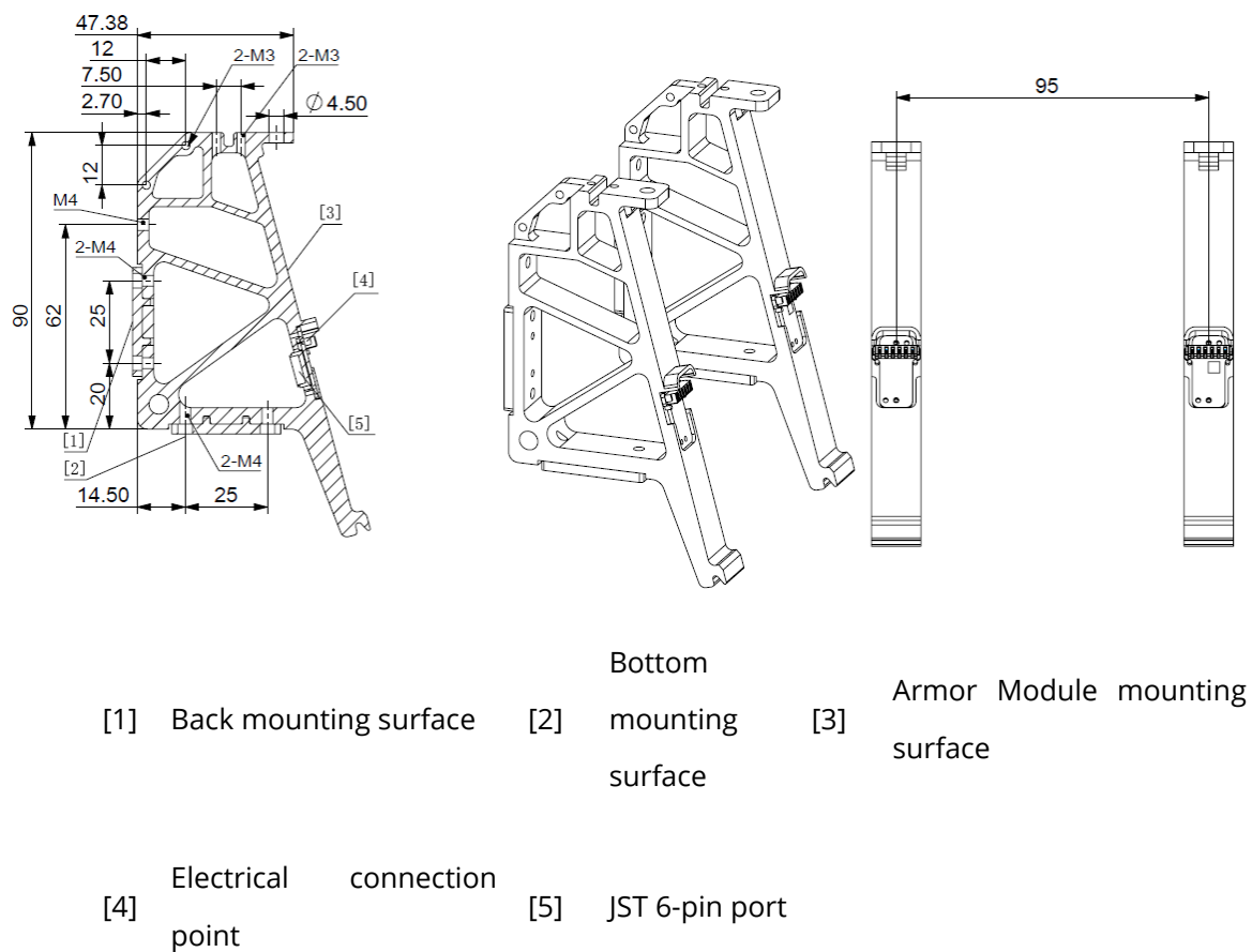
Figure 3-15 Designated Armor Support Frame
