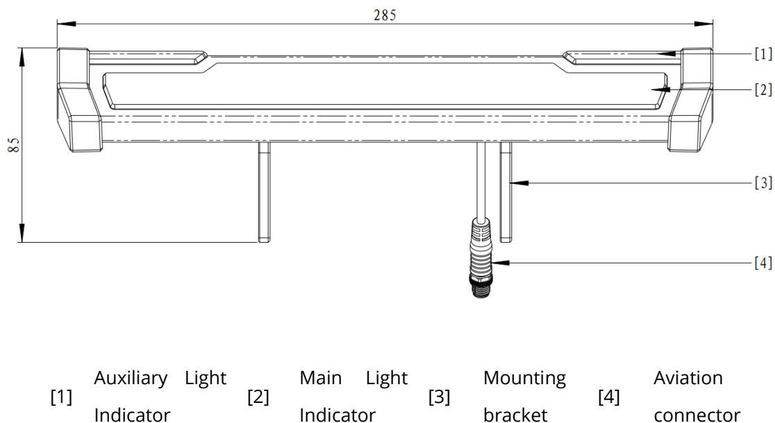
Figure 3-11 Light Indicator Module
