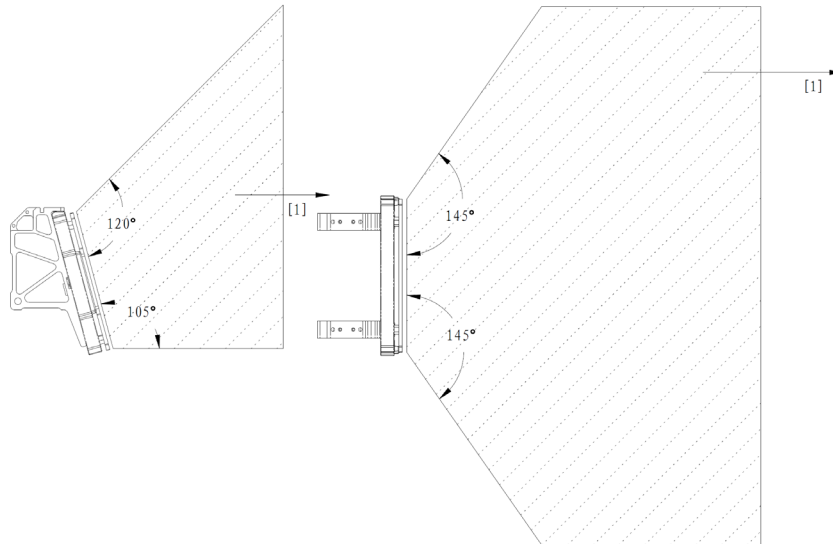
[1] Infinite extension
