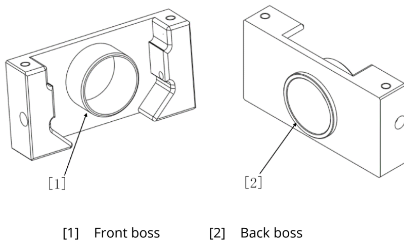
Figure 3-33 17mm Adapter Block
