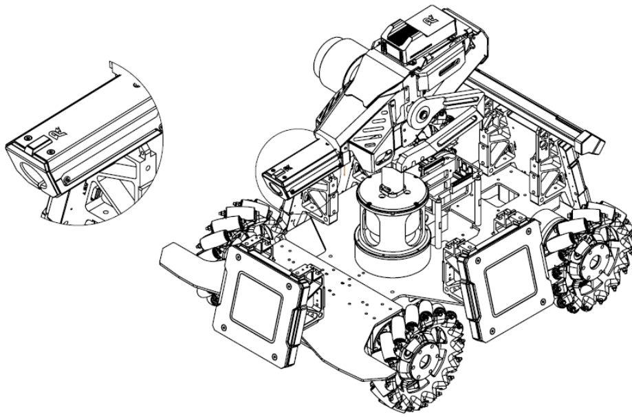
Figure 3-32 Speed Monitor Module Installation
