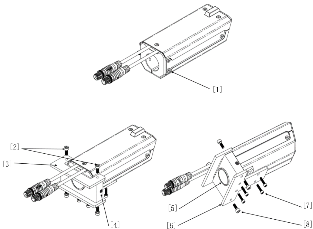
Figure 3-33 17mm Adapter Block
