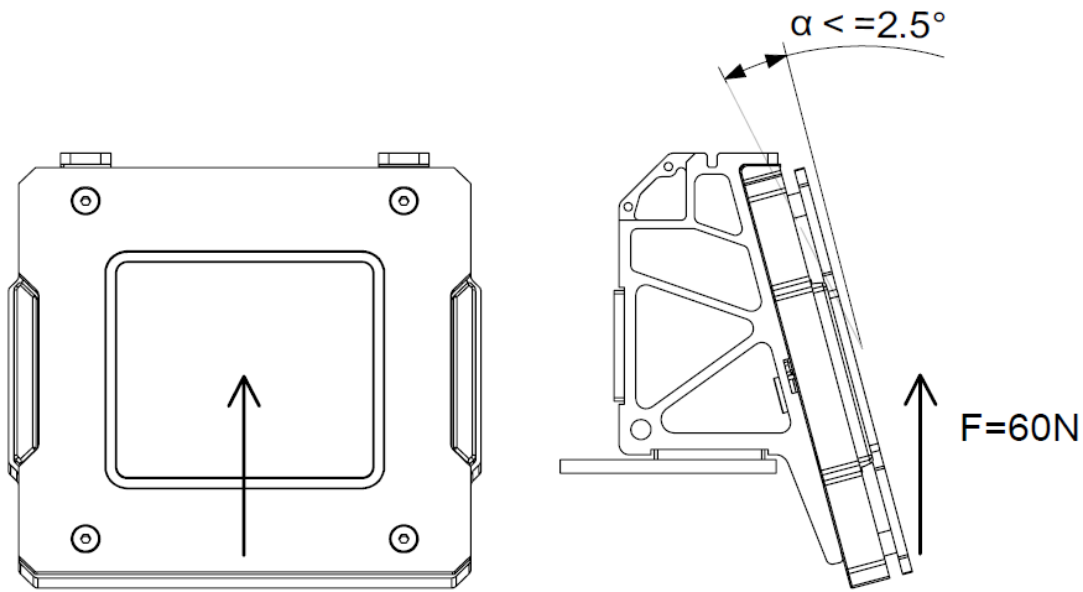
Figure 3-20 Forces on the Armor Module
