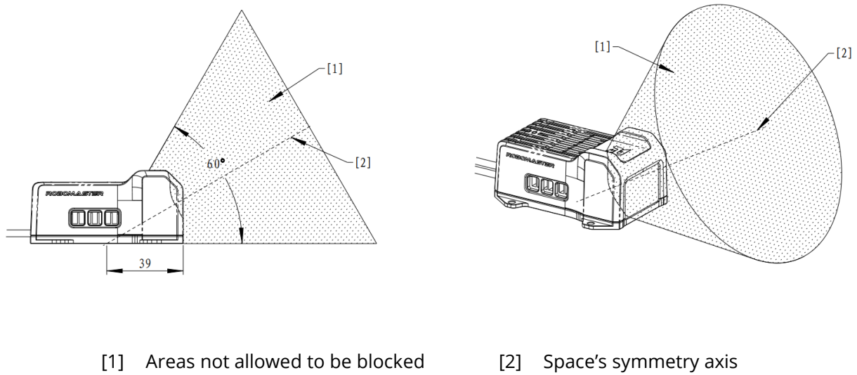
Figure 3-44 Prohibited Blockage Areas for Video Transmitter Module (Transmitter)
