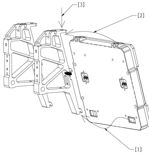
Figure 3-24 Armor Module Mounting
