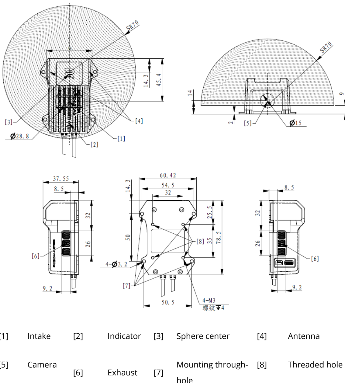
Figure 3-42 Video Transmitter Module (Transmitter)
