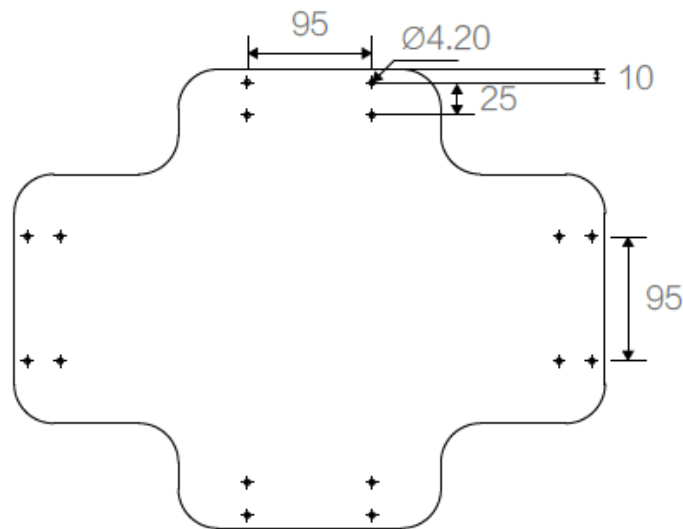
Figure 3-22 Chassis Reserved Holes
