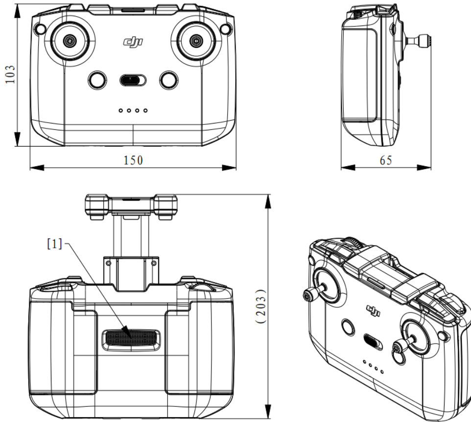
[1] Exhaust
