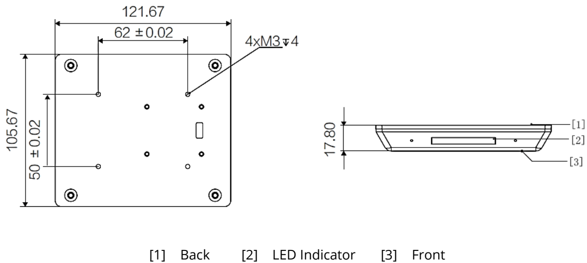
Figure 3-39 RFID Interaction Module
