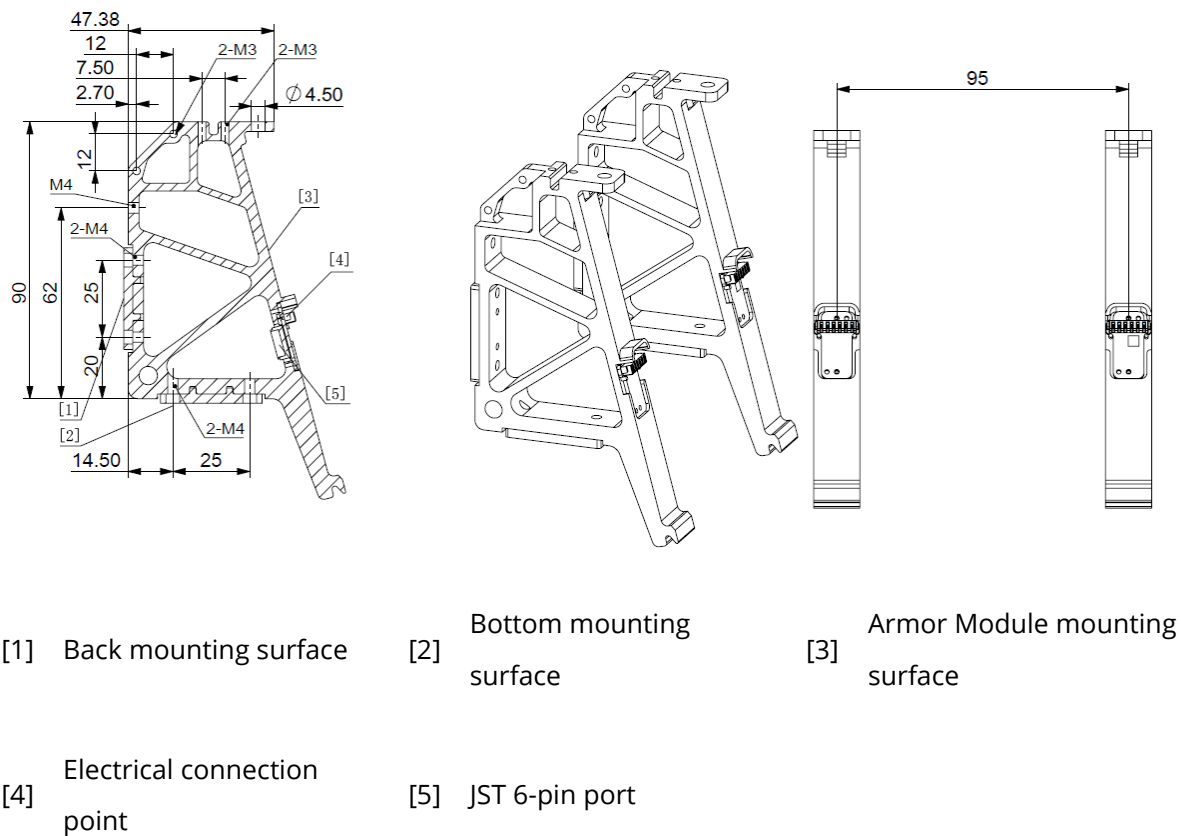
Figure 3-15 Designated Armor Support Frame
