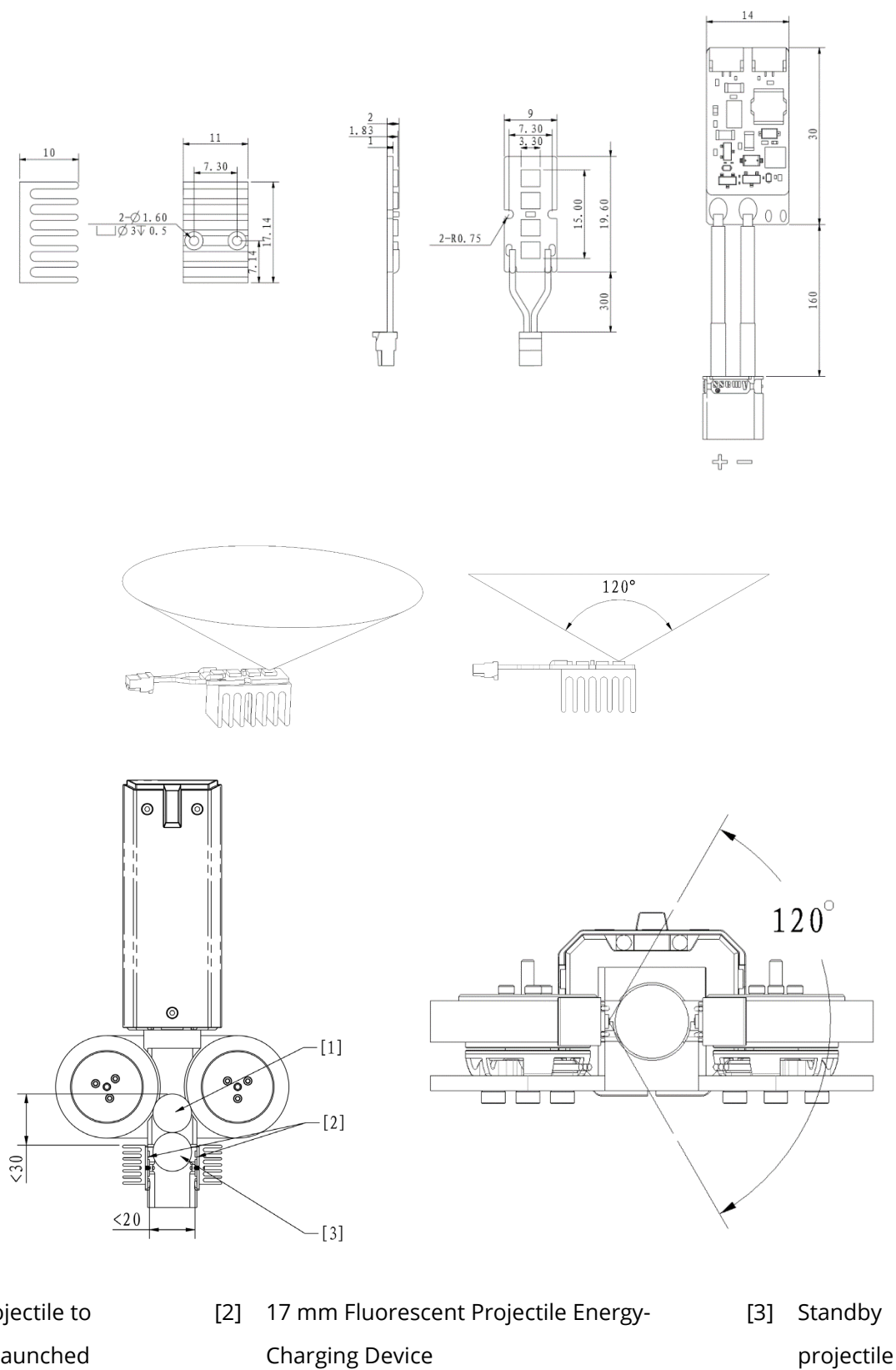
Figure 2-1 Mounting of 17 mm Fluorescent Projectile Energy-Charging Device
