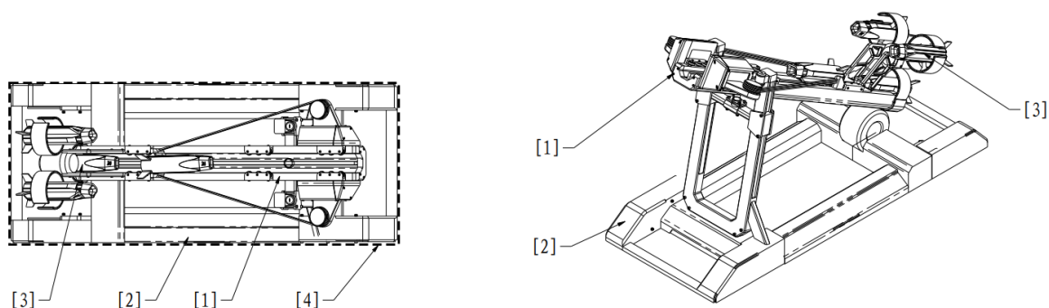
Figure 2-6 Dart System Size Limits
