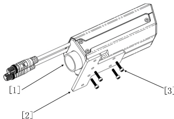
[1] Barrel [2] Self-produced part 1 [3] M2.5 screw
