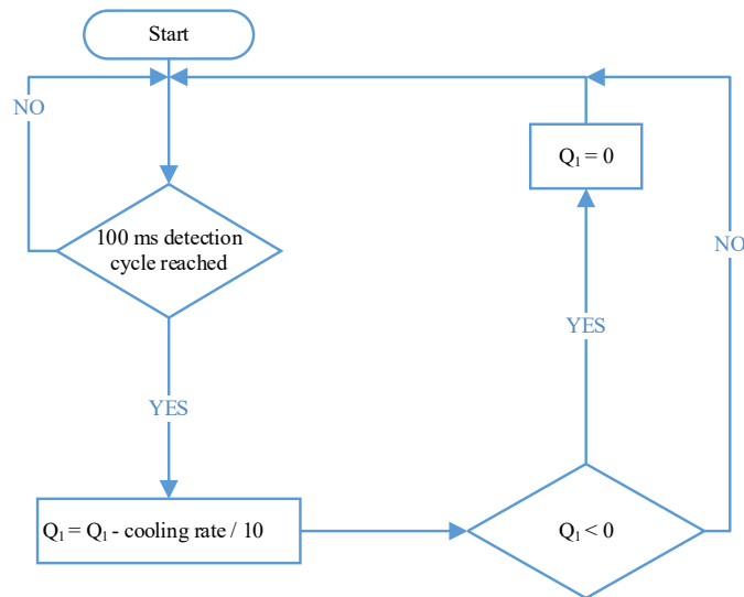
Figure 3-11 Barrel Heat Cooling Mechanism
