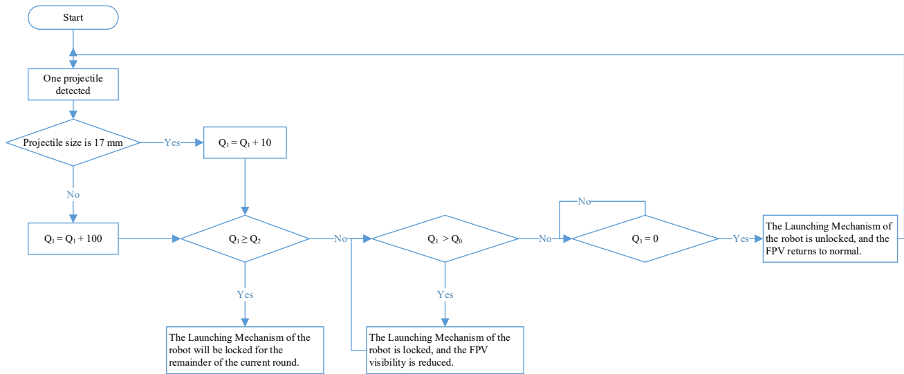
Figure 3-10 Penalty Mechanism for Exceeding the Barrel Heat Limit
