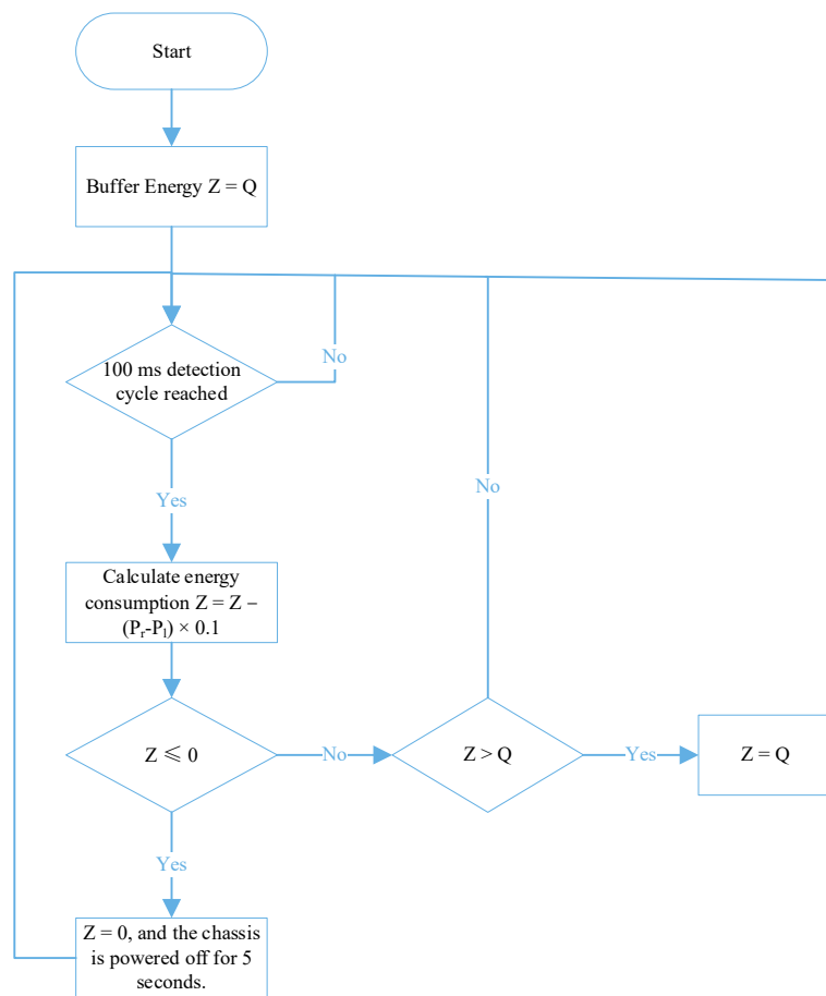
Figure 3-12 Robot Chassis Power Detection and Penalty for Exceeding Limit
