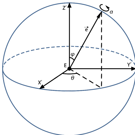
Figure 5-5 Spherical Coordinate System
