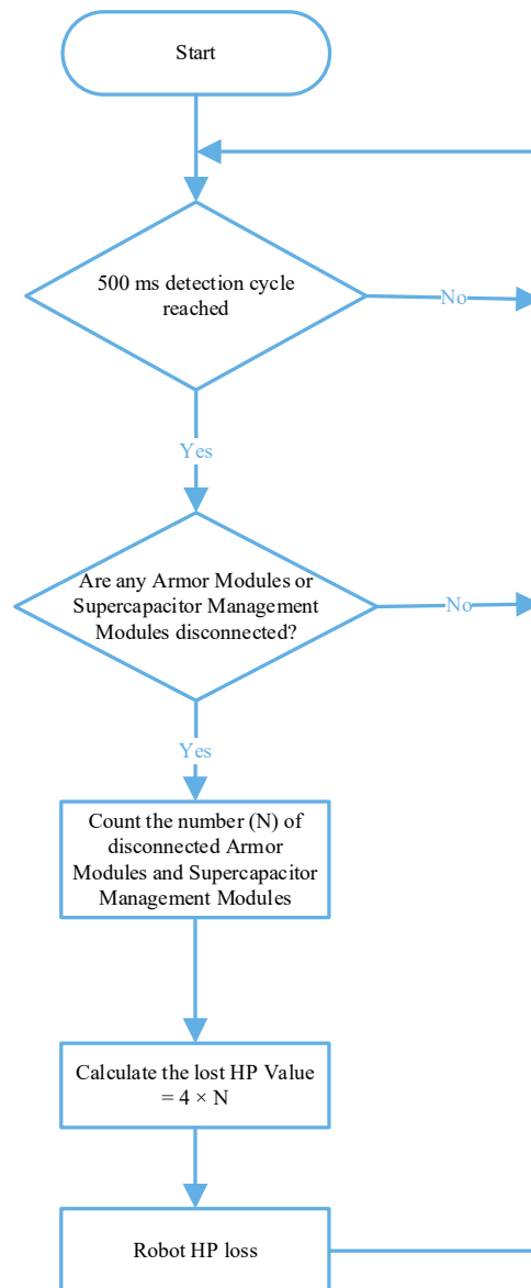
Figure 3-13 HP Loss Mechanism for Armor Module and Supercapacitor Management Module Disconnection
