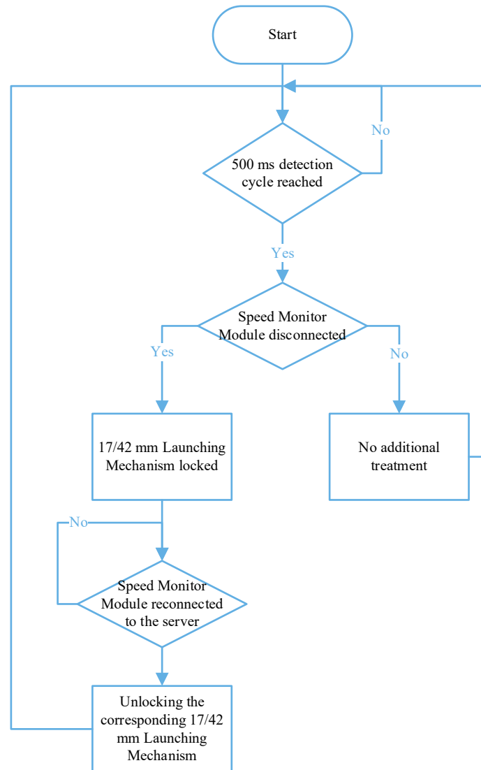
Figure 3-14 Power-off Mechanism for Speed Monitor Module Disconnection
