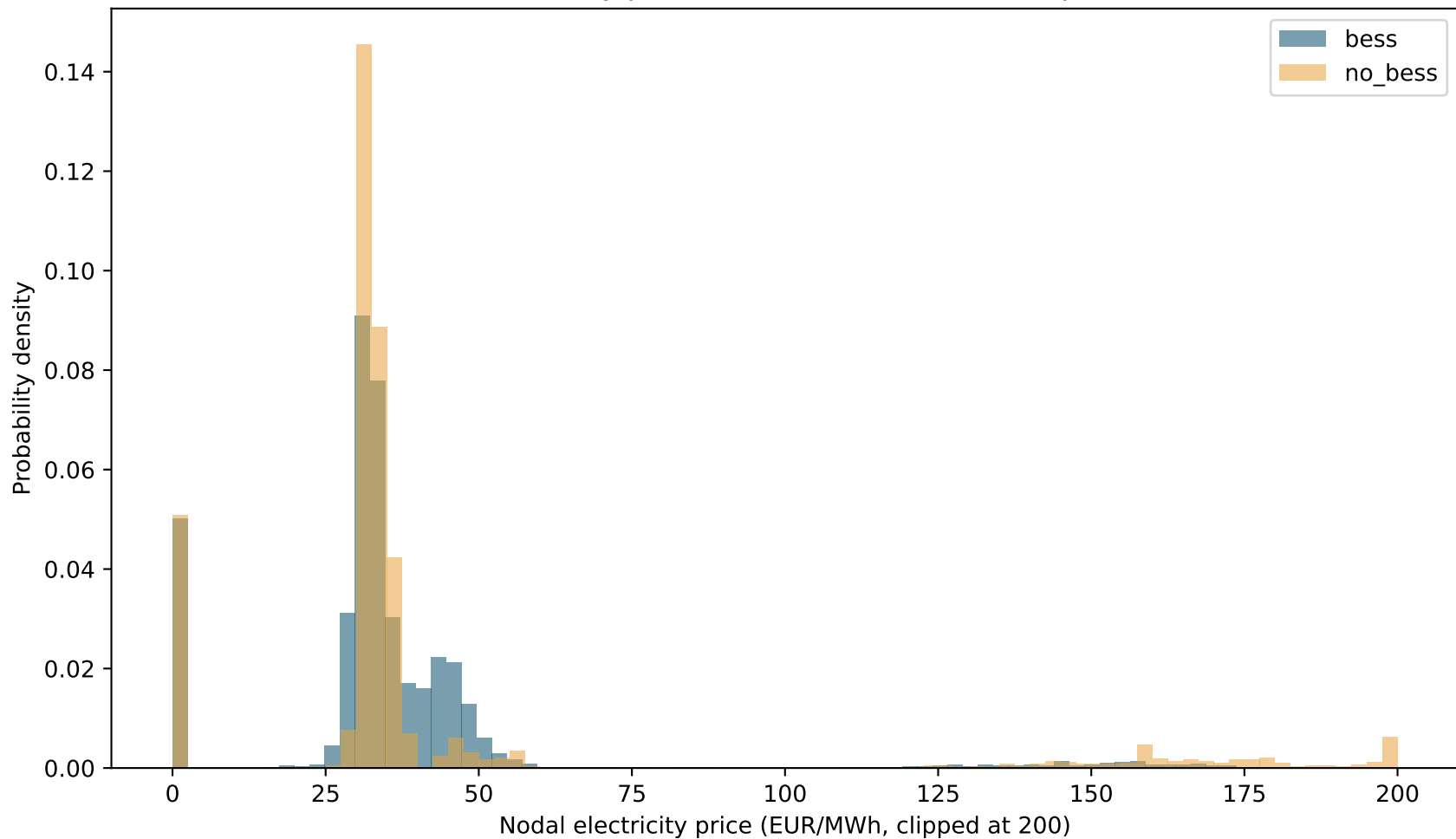
Electricity price distribution -- 2050, ll=vopt
