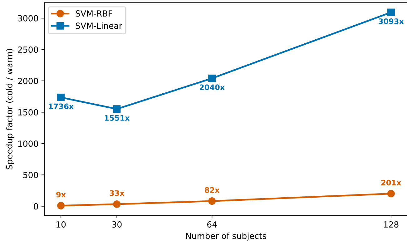
Cache Speedup Scales with Dataset Size
