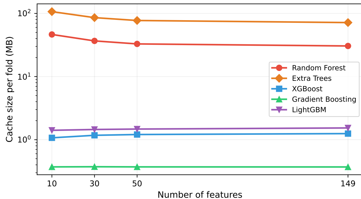
Cache Size vs. Feature Count
