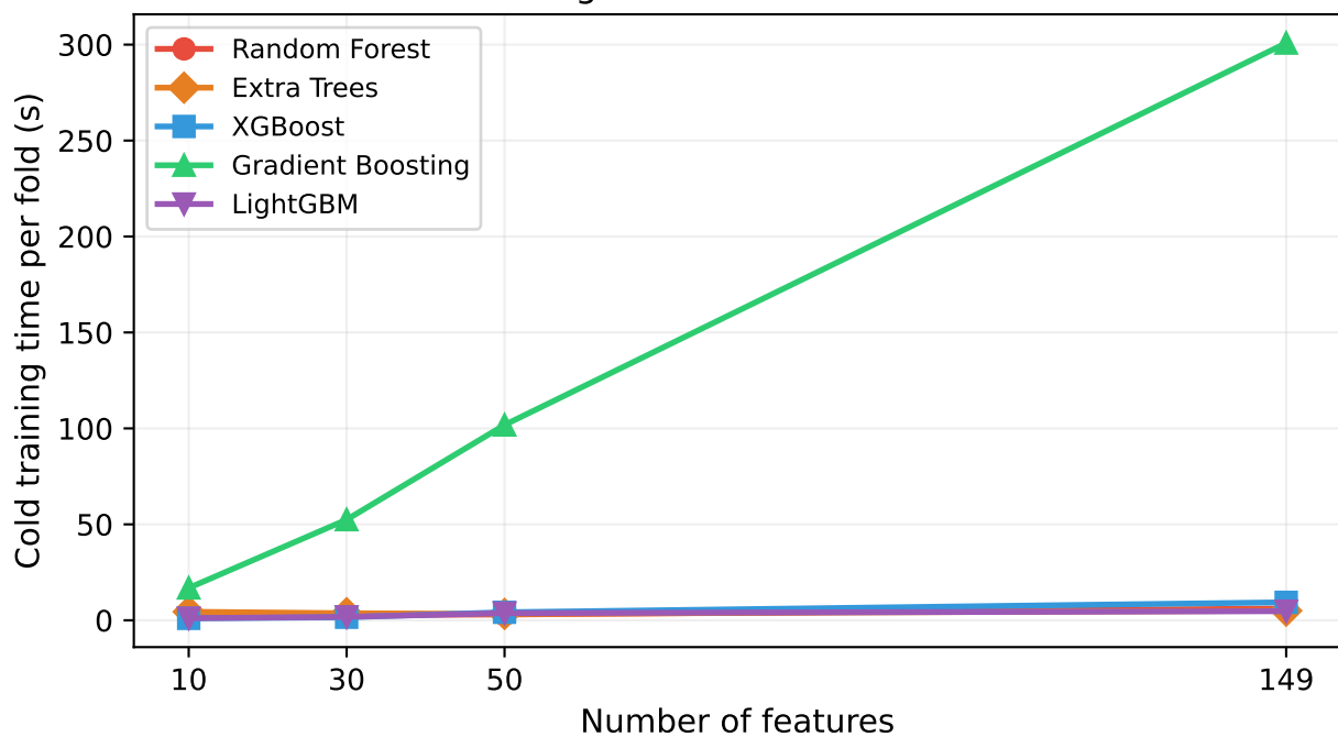
Training Time vs. Feature Count
