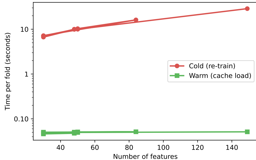
XGBoost
