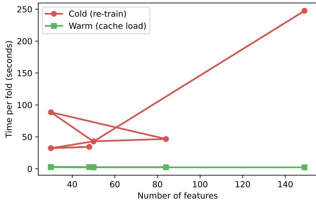
Random Forest
