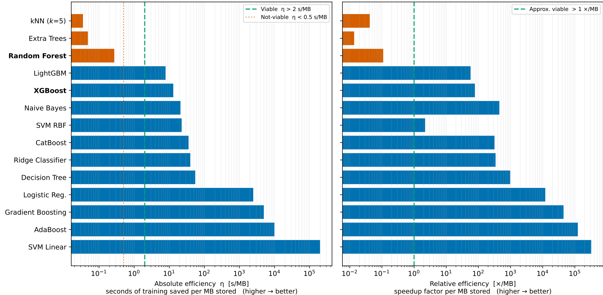
Absolute Efficiency ( \eta )
