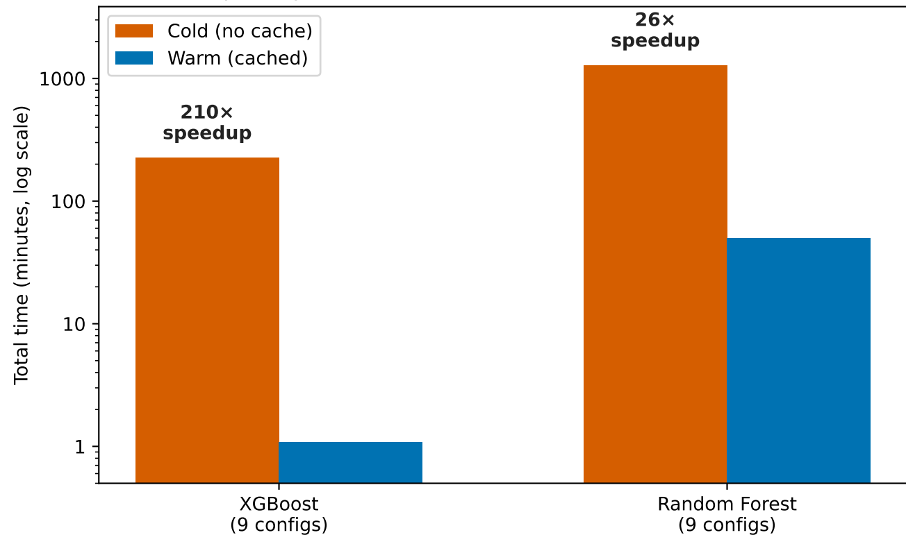
Cache Speedup: Cold Start vs. Cached Execution (128 LOSO folds)
