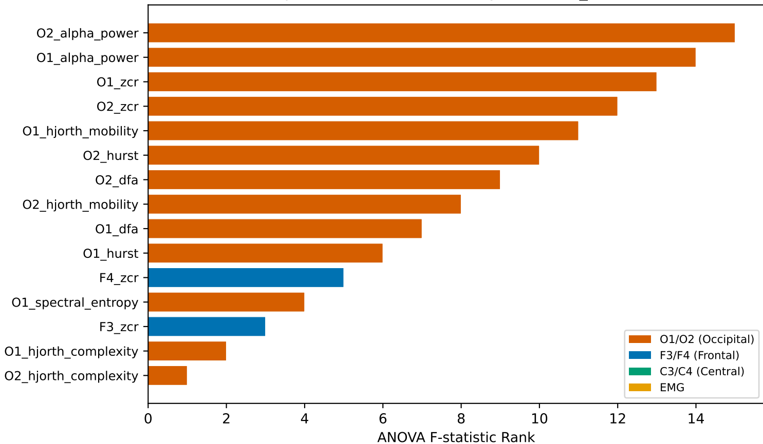
Top 15 Features Selected by ANOVA (f_classif)
