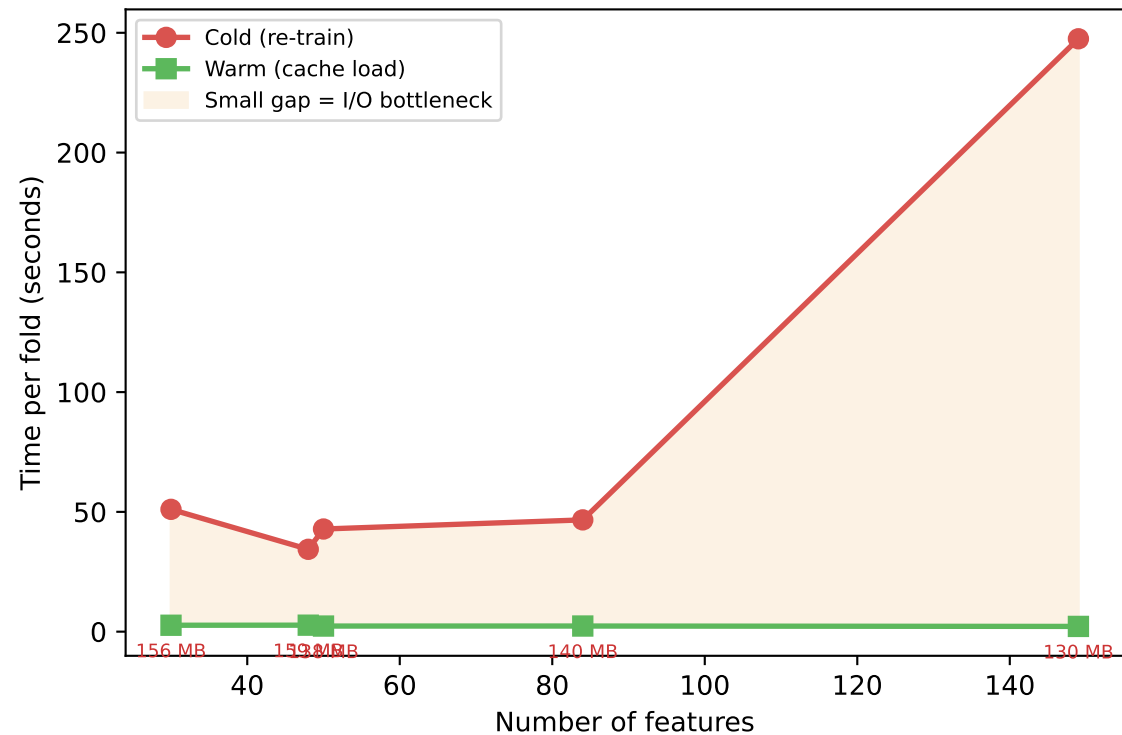
Random Forest — ~131 MB/fold, loads in 2.5s
