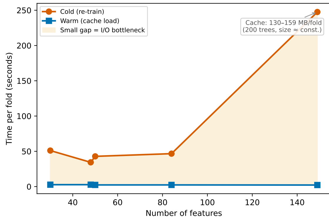
Random Forest — ~145 MB/fold, loads in 2.5s
