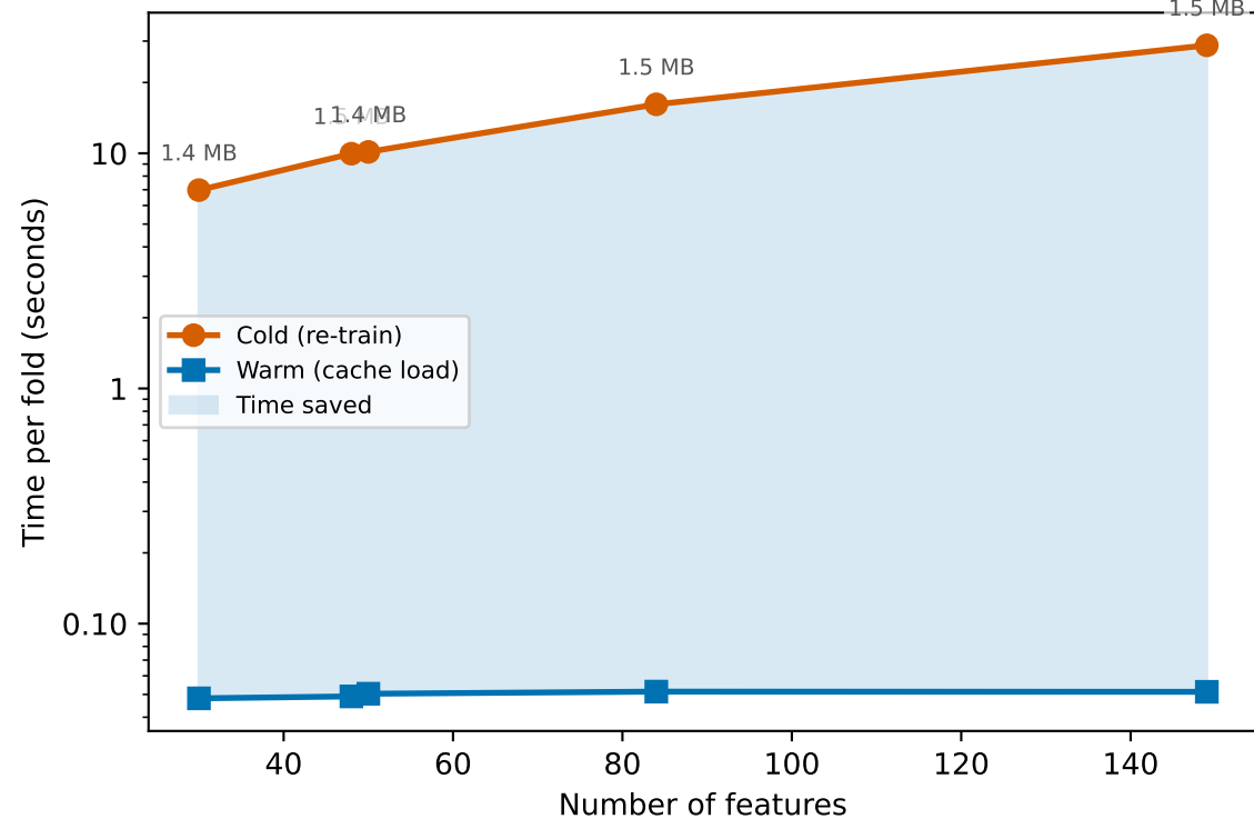
XGBoost — ~1.5 MB/fold, loads in 0.05s
