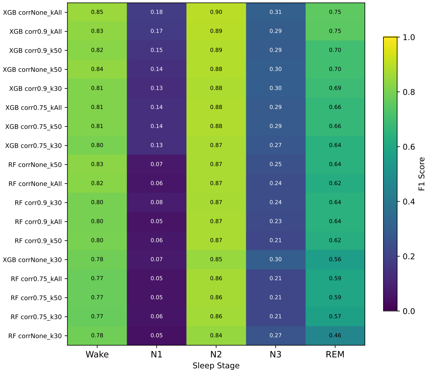
Per-Class F1 Score Across All 18 Configurations
