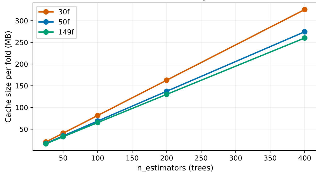
Cache Size Grows Linearly with Trees
