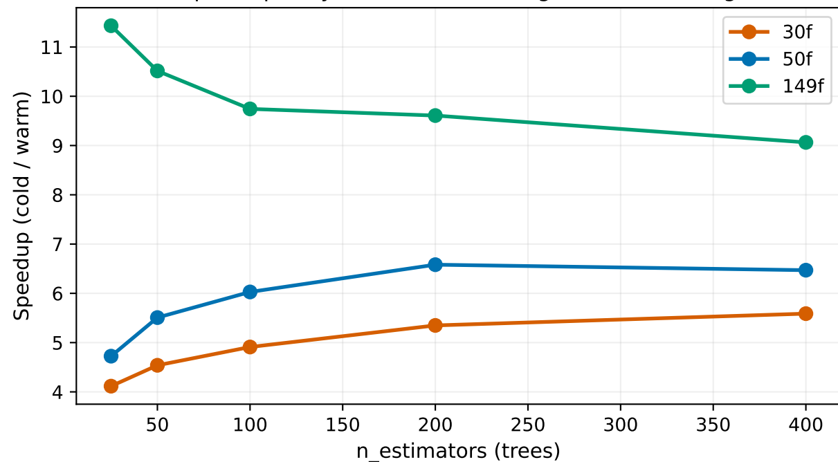
Speedup Stays Low (~5-11x) Regardless of Config
