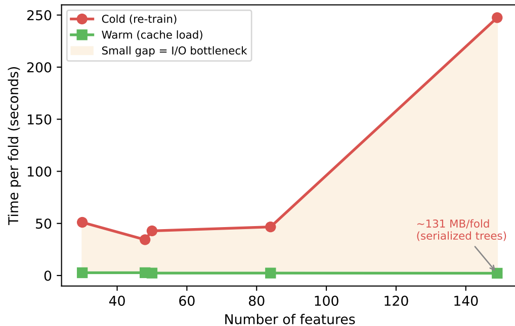
Random Forest — cache load ~2.5s (131 MB I/O)
