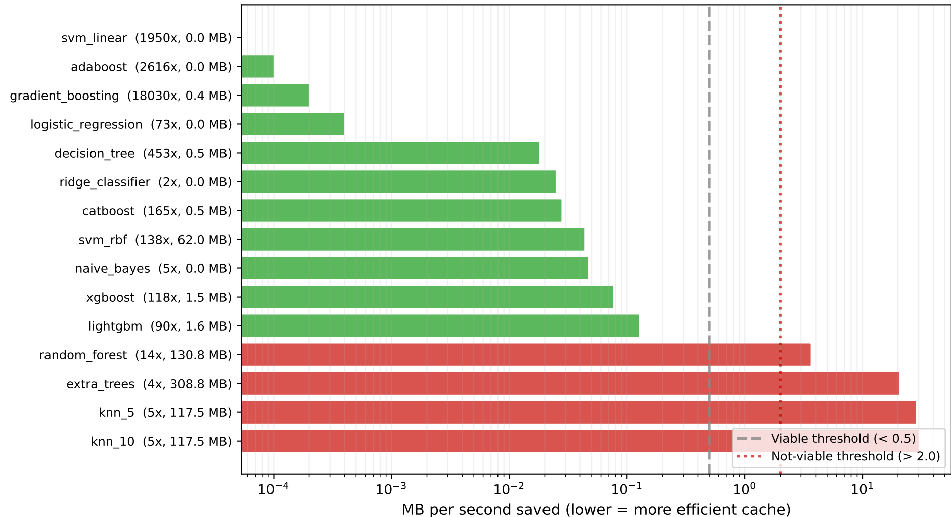
Cache Viability Metric: Storage Cost per Second of Compute Saved Green = viable, Red = not viable (I/O dominates)
