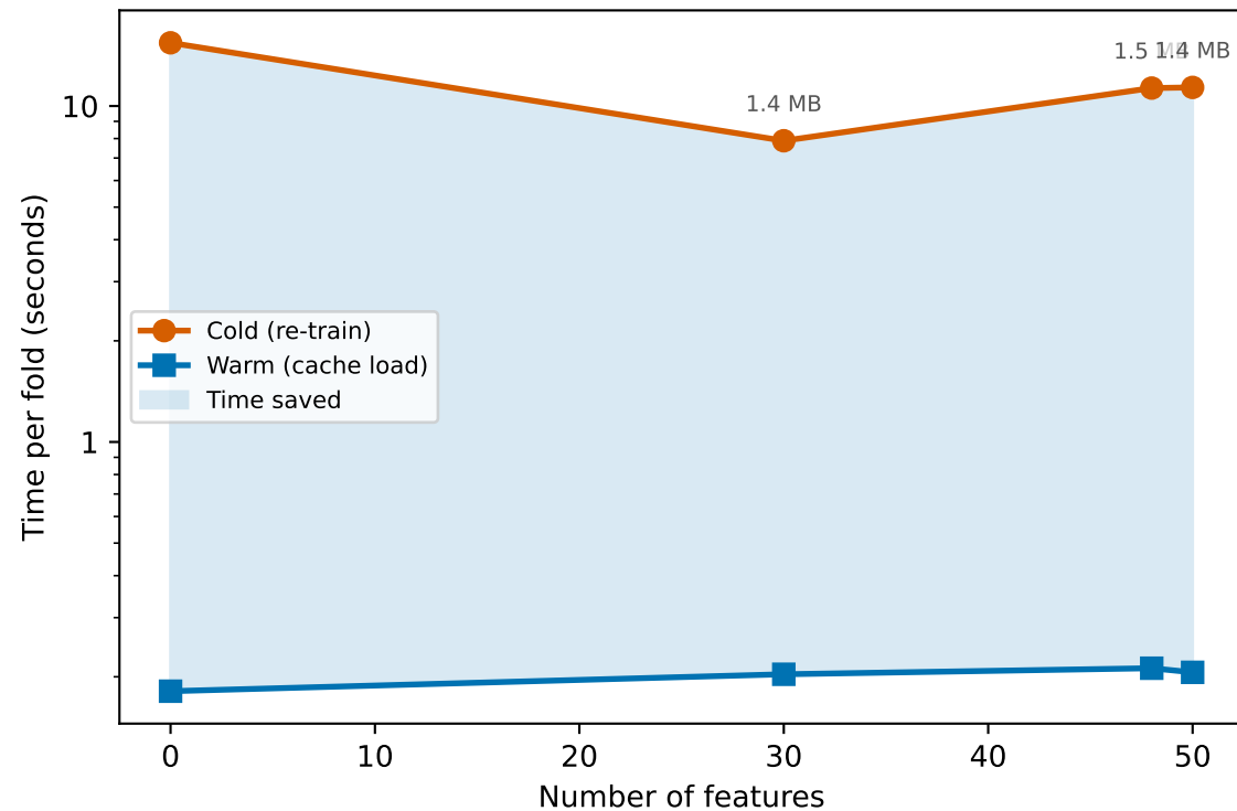
XGBoost — ~1.5 MB/fold, loads in ~0.2s
