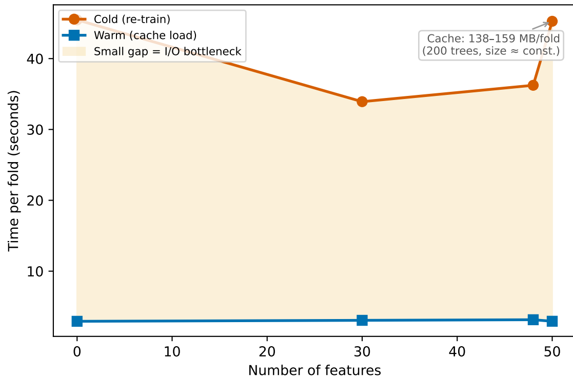
Random Forest — ~151 MB/fold, loads in ~3s
