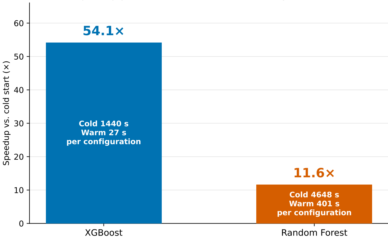
Cache Speedup per Model (median across 9 configs, 128 LOSO folds)
