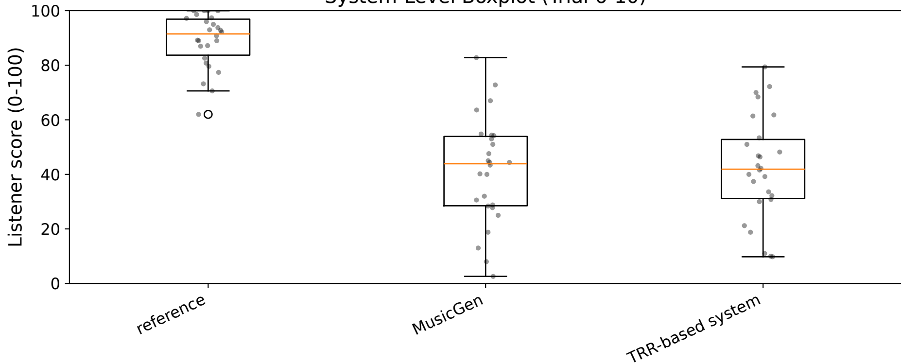
System-Level Boxplot (Trial 6-10)
