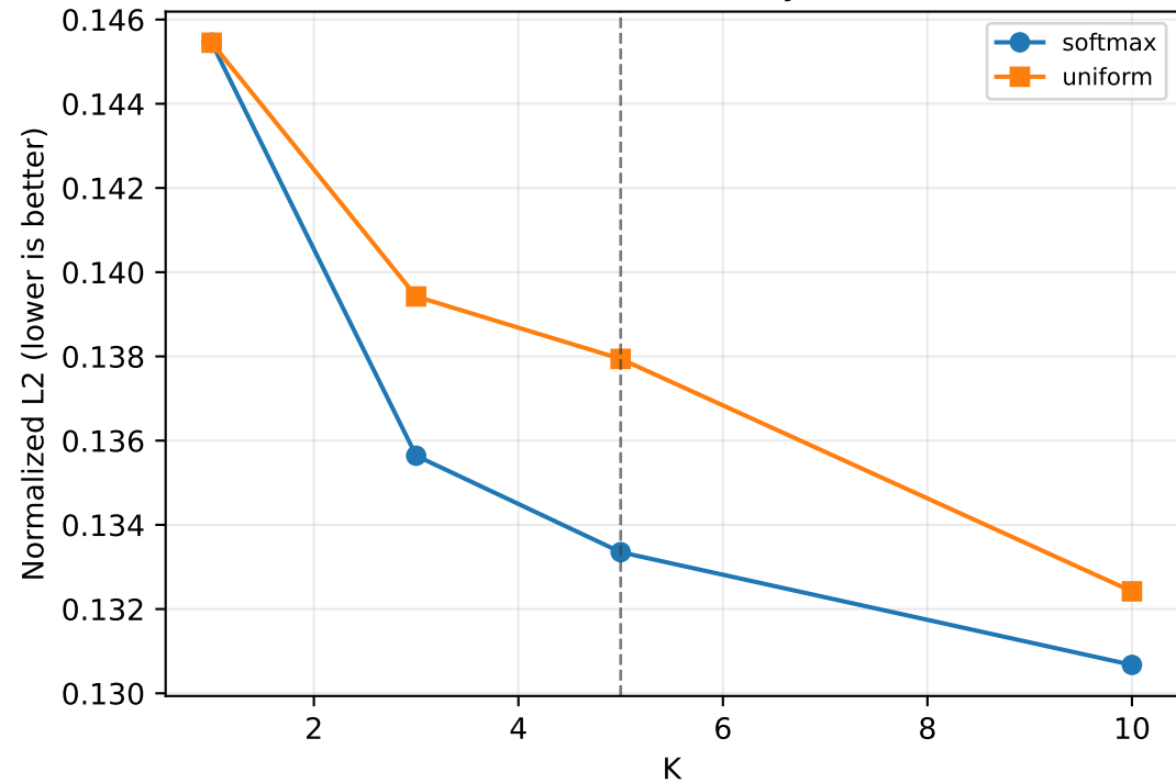
EPR Sensitivity
