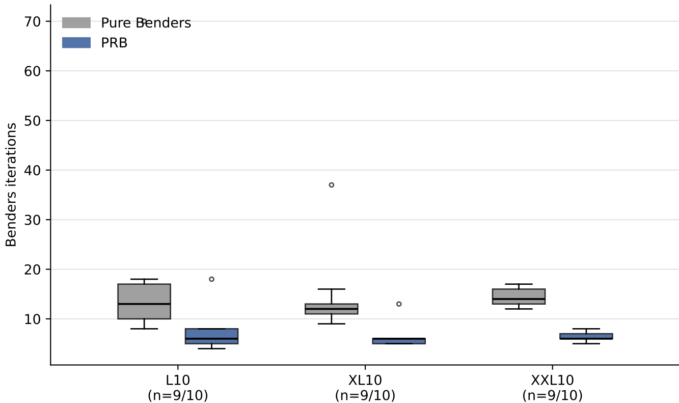
Benders iteration counts across controlled network scales
