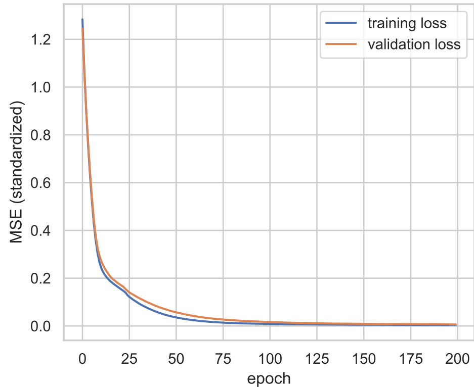
Baseline MLP — learning curves
