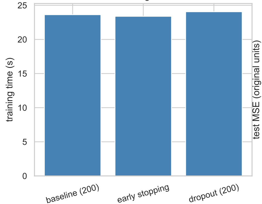
Training time
