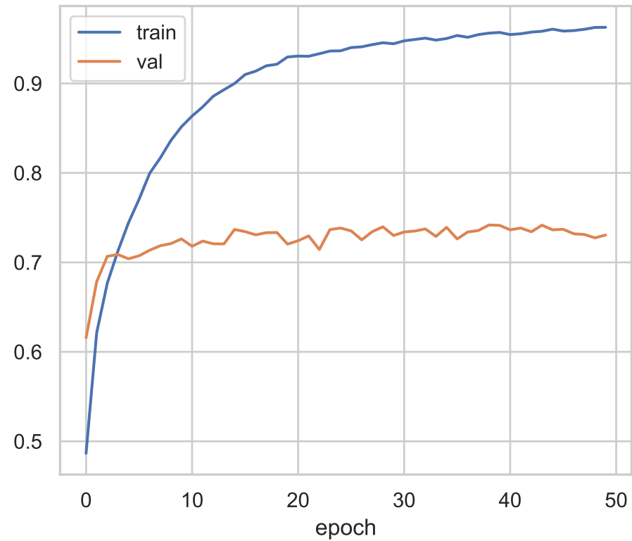
CNN accuracy
