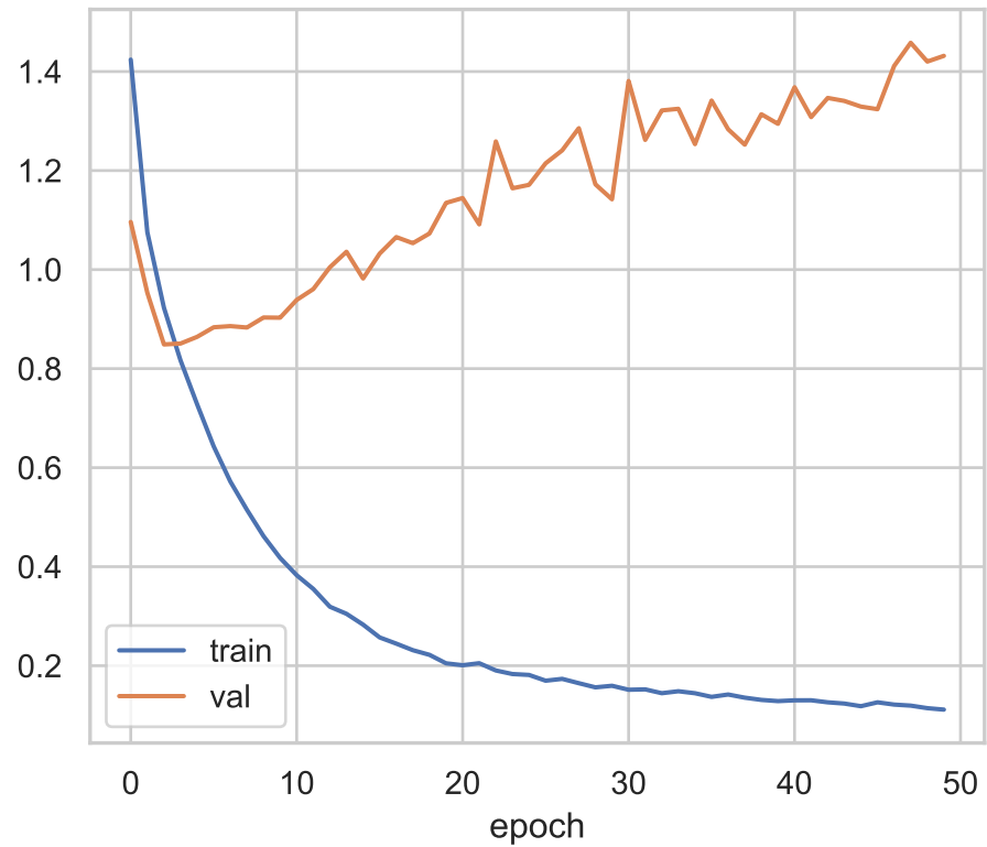
CNN loss
